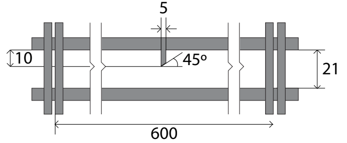
FIGURE 1: LATERAL VIEW OF THE FENCE [mm]
