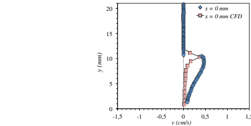
FIGURE 11: VERTICAL VELOCITY PROFILE COMPONENTS AT DIFFERENT DISTANCES FOR THE FENCE
