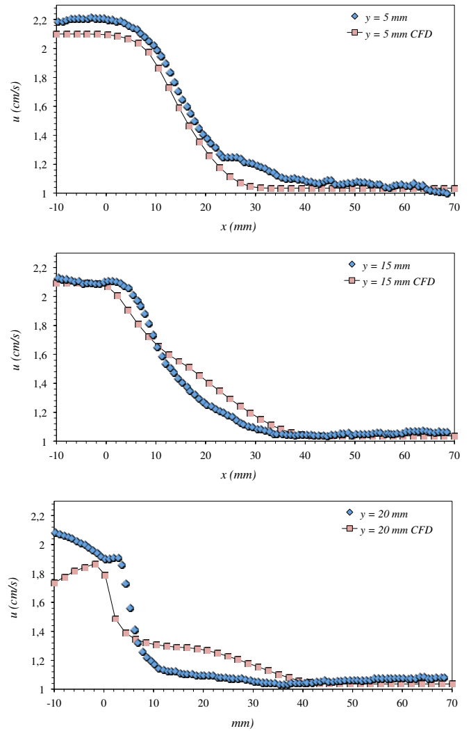
FIGURE 14: AXIAL VELOCITY IN THE VICINITY OF THE HALF-SUDDEN EXPANSION AT DIFFERENT HEIGHTS
