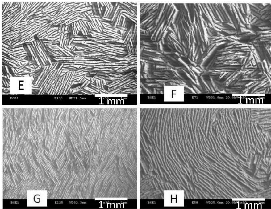
Figure 6. SEM micrographs of cross section parallel (A–D) and perpendicular (E–H) to the freezing direction of freeze cast anisotropic porous specimens as a function of processing parameter (28 wt. % alumina). (A,C,E,G) without binder; (B,F) with 3 wt. % of binder; (D,H) with 6 wt. % of binder. (C,G) frozen at 20 K/min, others at 1 K/min.
