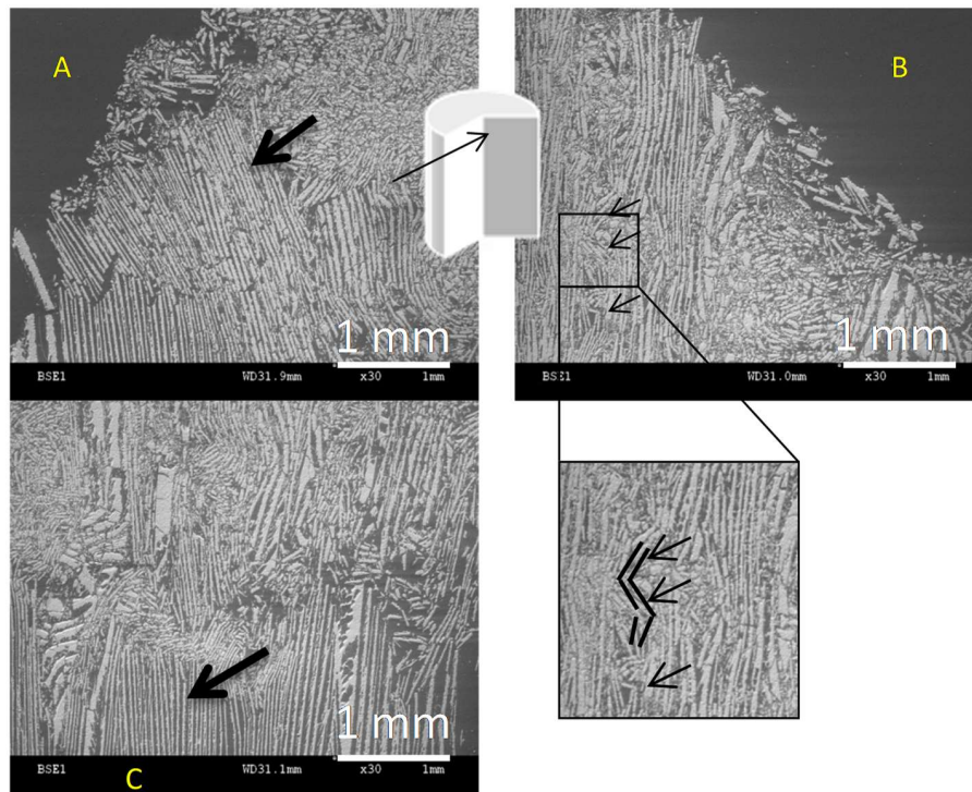
Figure 9. SEM micrographs of a specimen processed at 1 K/min, from a slurry with 28 vol. % of alumina and 3 wt. % of binder. (A) top left; (B) top right and (C) centre of the specimen.
