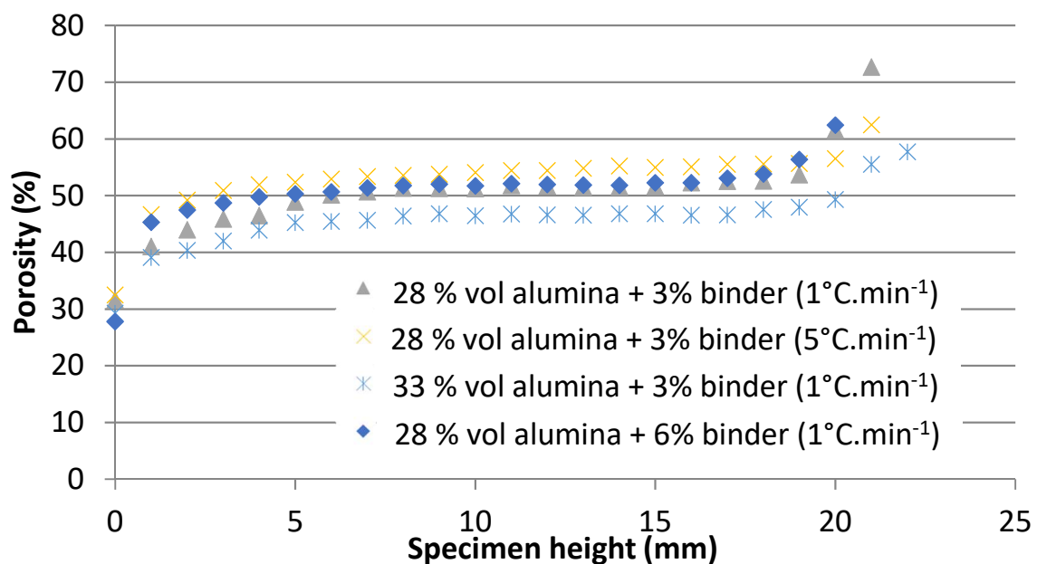
Figure 12. Porosity gradient measurement of specimens processed under different conditions. Each measurement point is an average value of Y1, Y2 and Y3.
