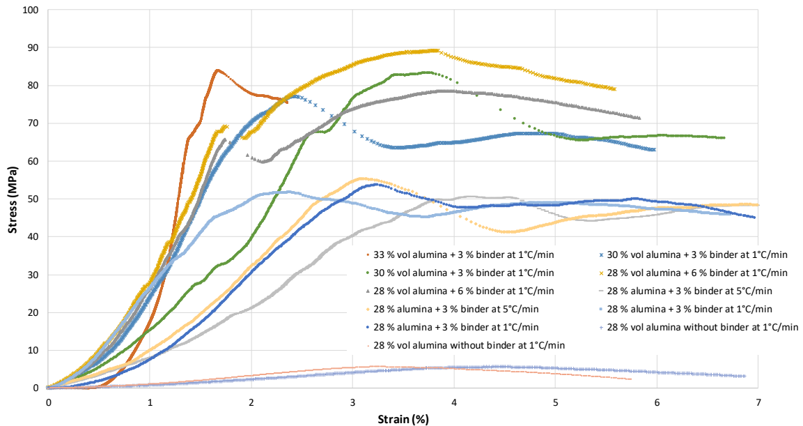
Figure 7. Stress measurement of anisotropic porous alumina specimen processed at different parameters.
