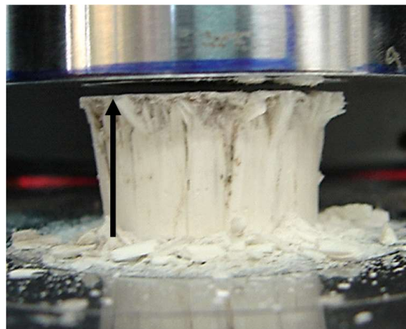
Figure 8. Image of porous alumina specimen during compressive test. The dark arrows represent the freezing direction during the freeze casting.
