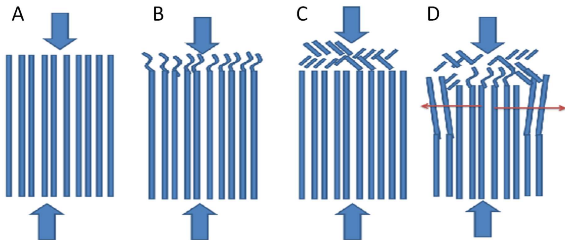
Figure 11. Schematic of rupture mode of a freeze cast specimen during the compression test. (A) at start of load application; (B) lamellae deformation when the load increases; (C) lamellae fracture. By further increase of the load, lamellae pieces filled the pore and push the other lamellae to obtain a trapezoidal shape (D).
