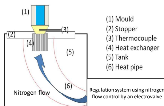
Figure 1. Schematic of the freeze casting device [26].
