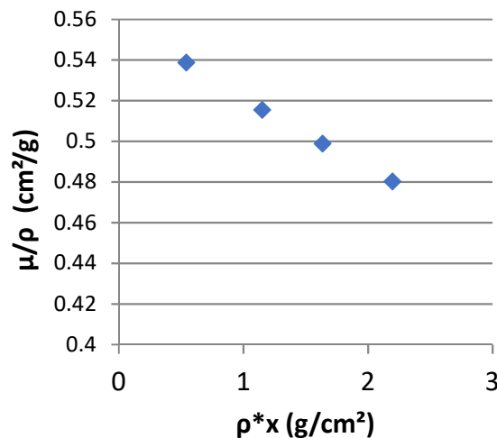
Figure 5. Mass absorption coefficient as a function of the mass thickness.
