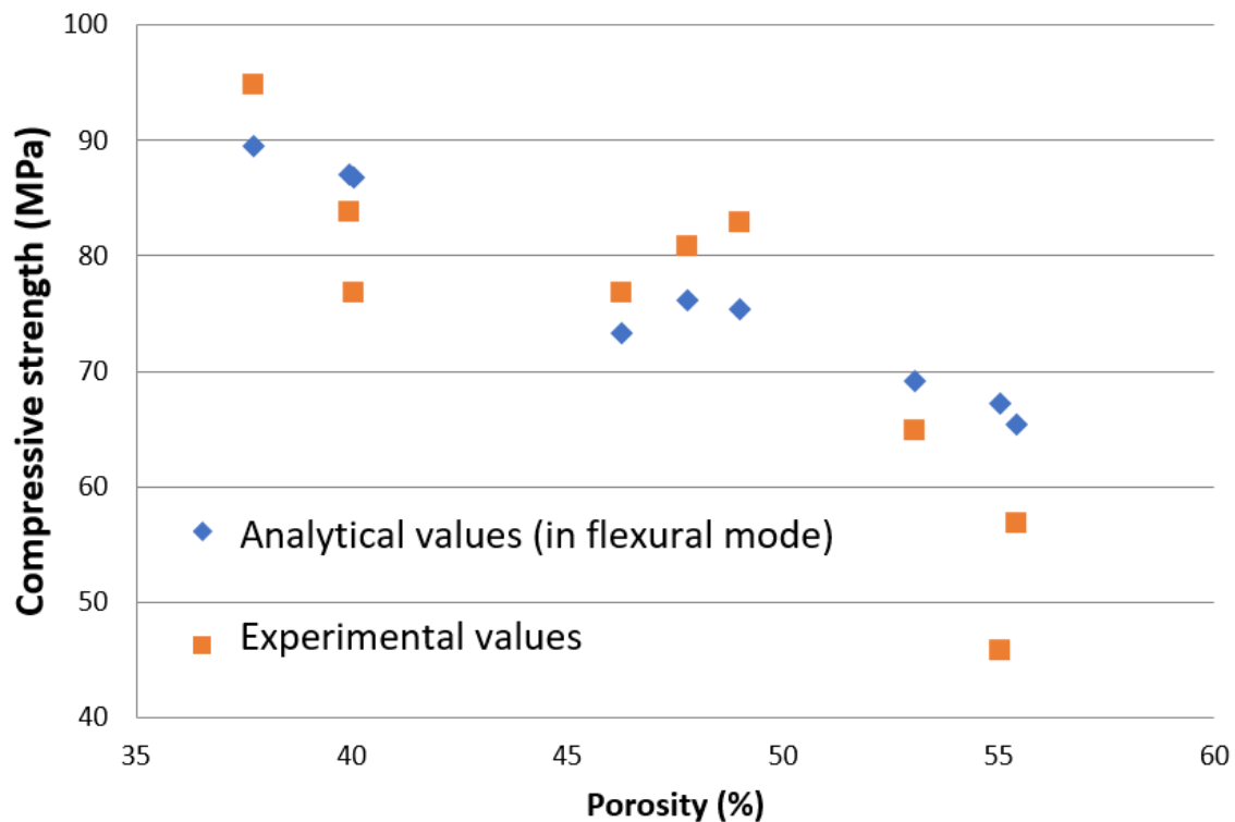
Figure 13. Compressive strength of porous anisotropic alumina as a function of the porosity level. Comparison of experimental and analytical values for the specimens characterised in Table 3.
