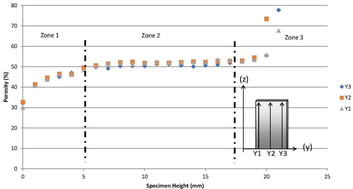
Figure 10. Porosity gradient measurement along z axis of a specimen: slurry containing 28 vol. % alumina + 3 wt. % binder and frozen at 1\text{ K}/\text{min} .
