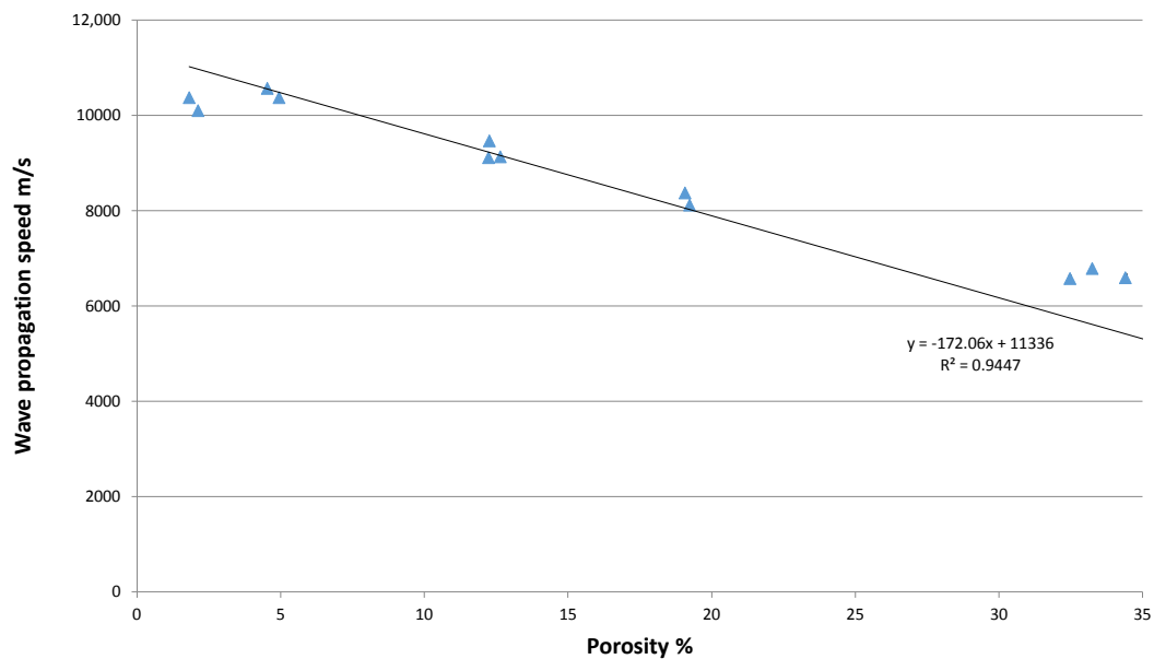
Figure 3. Standard curves of ultrasound wave propagation speed as a function of porosity for isotropic porous alumina.
