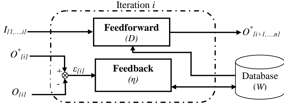
Fig. 5. Iterative and sequential reinforced learning structure.
