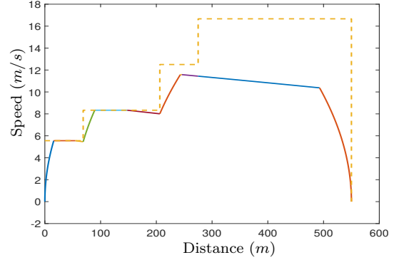
Fig. 3. The speed trajectory of the fast trip time and his characteristics T_i = 70 , E = 4.7801e^6
