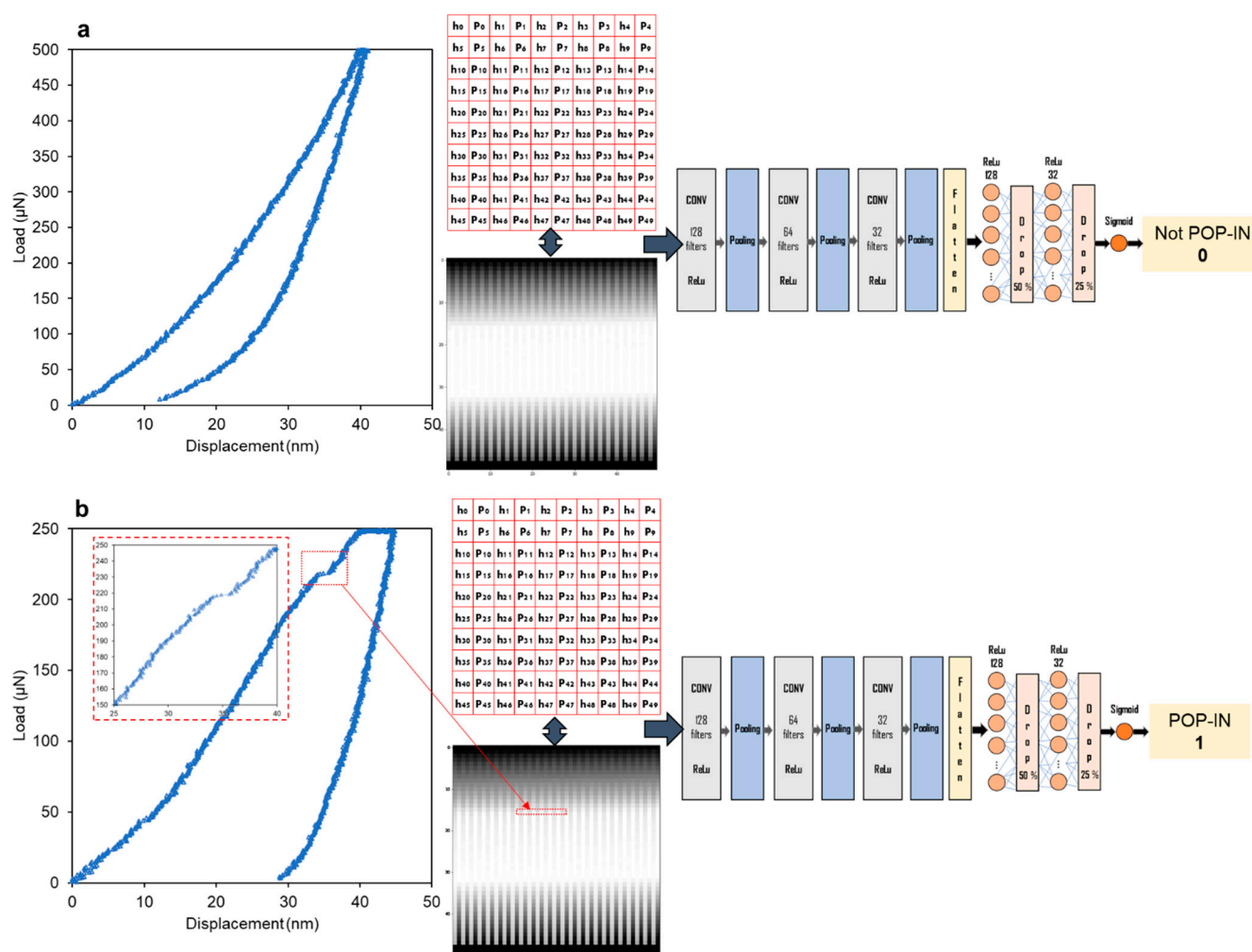
Figure 5. CNN implementation workflow: load–displacement curves (a. typical loading path, b. pop-in) are converted into matrices (“images” in grayscale) which are the inputs to pass to the CNN model, which give an output equal to 0 for no pop-in and 1 for pop-in events. The numerical matrices are just for illustration and do not represent the model’s 50 \times 50 matrices used as input.
