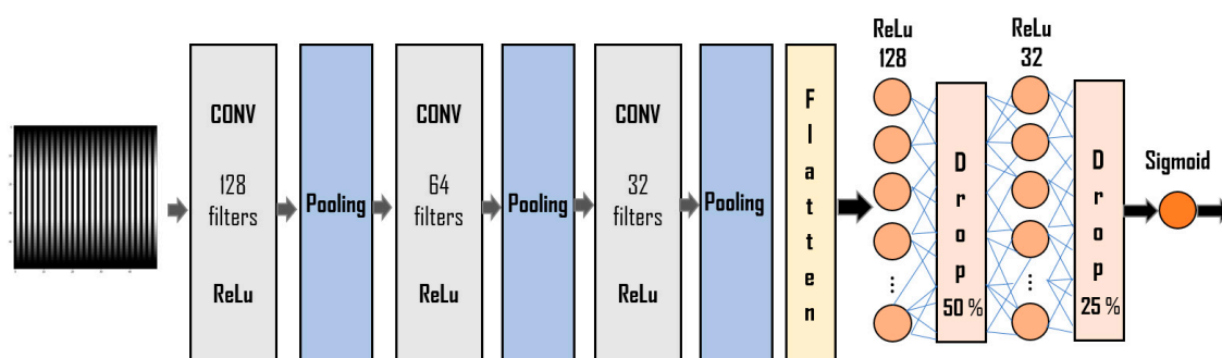
Figure 3. The architecture of the CNN model implemented to classify curves with pop-in and without pop-in events.
