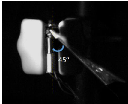
Figure 14: Diagram of wing observation experiment set-up
