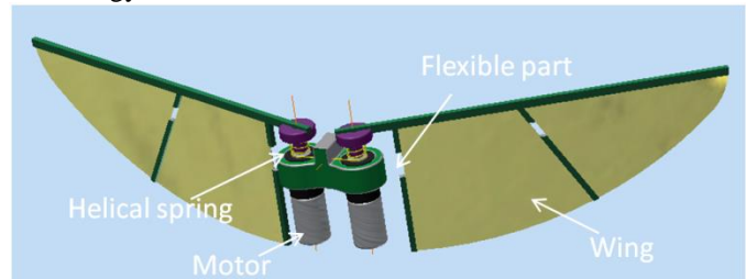
Figure 1: MAV concept
