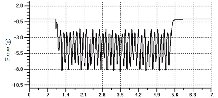
Figure 16: Force measurement
