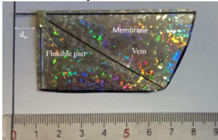
Figure 13: Fabricated Wing
