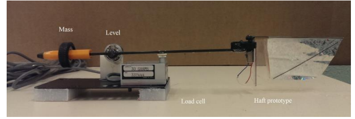
Figure 15: Lift measurement set-up
