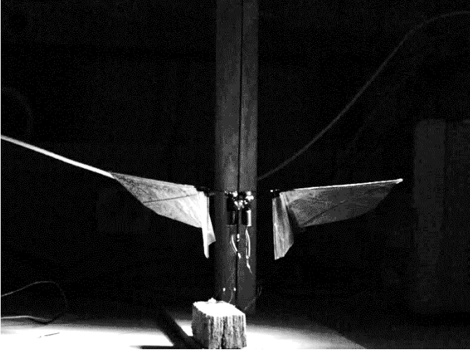
Figure 17: Take-off demonstration
