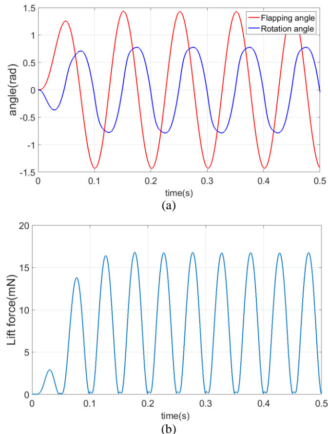
Figure 11: Dynamic simulation of a proper wing trajectory (a) and resulting lift force (b)
