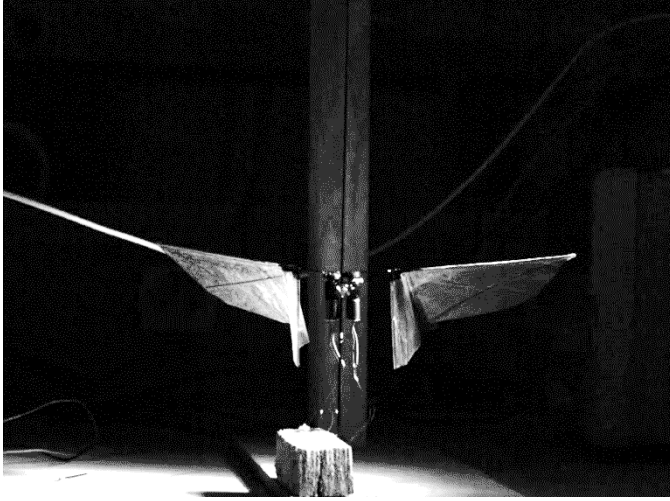
Figure 17: Take-off demonstration
