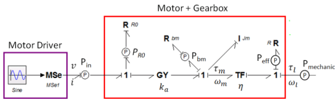
Figure 3: Motor driver and motor with gearbox blocks
