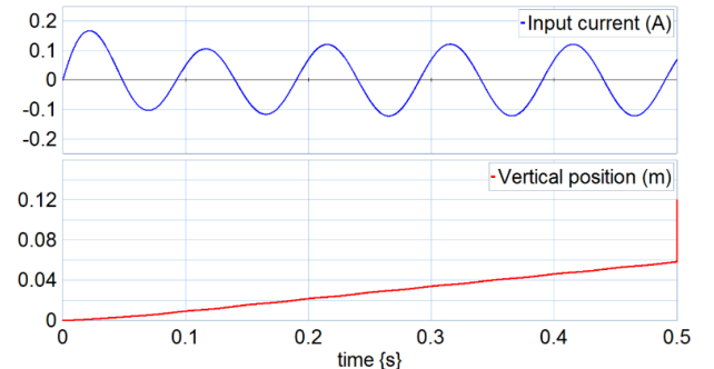
Figure 12: Simulation of vertical take-off
