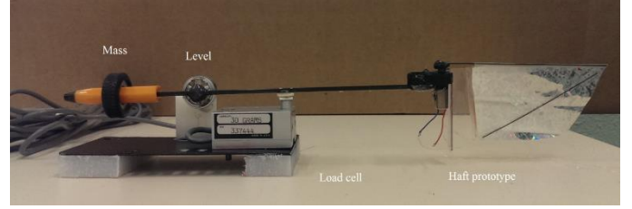
Figure 15: Lift measurement set-up
