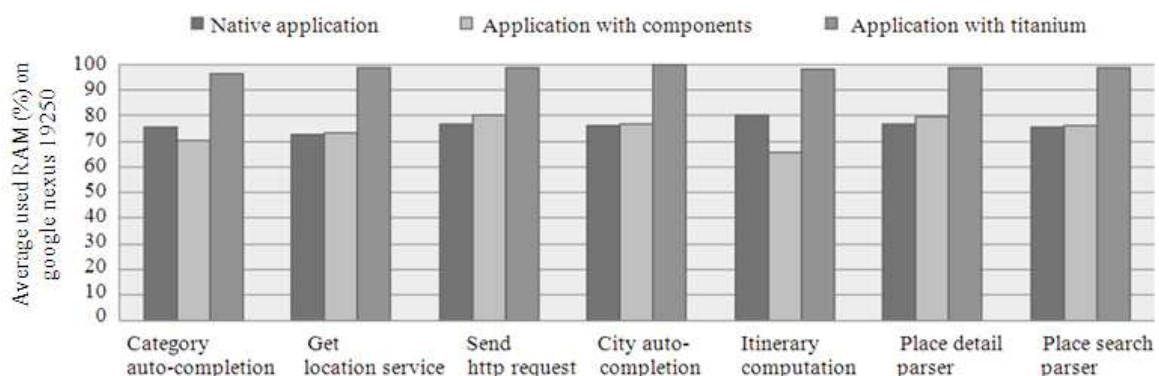
Fig. 14. Used RAM for each LocaPlace application version after several tasks execution
