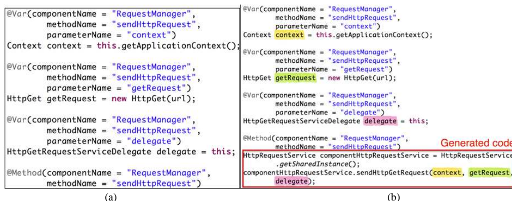
Fig. 11. (a) Necessary annotations to call (b) Generated code to call the sendHttpRequest method with native language on Android (Java)
