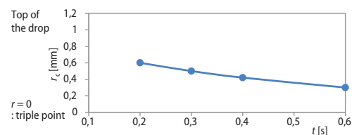
Figure 12. Evolution of the position of the transition point c at interface liquid-gas (from triple point to top of drop) as function of time: T_h = 70 \text{ }^\circ\text{C} , T_0 = 22 \text{ }^\circ\text{C} , H = 40\% and \theta_0 = 65^\circ
