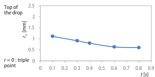
Figure 8. Evolution the position of maximum condensation point c at interface liquid-gas (from triple point to top of drop) as function of time: T_h = 80\text{ }^\circ\text{C} , T_0 = 22\text{ }^\circ\text{C} , H = 50\% and \theta_0 = 80\text{ }^\circ
