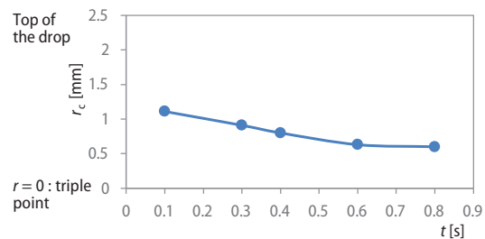
Figure 8. Evolution the position of maximum condensation point c at interface liquid-gas (from triple point to top of drop) as function of time: T_h = 80 °C, T_0 = 22 °C, H = 50\% and \theta_0 = 80 °
