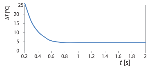
Figure 11. Evolution of temperature difference at liquid-gas interface vs. time: T_h = 70 \text{ }^\circ\text{C} , T_0 = 22 \text{ }^\circ\text{C} , H = 40\% and \theta_0 = 65^\circ
