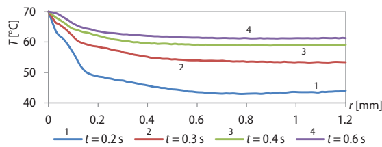
Figure 10. Variations in temperature at liquid-gas interface (from triple point to top of drop) of different times: T_h = 70 \text{ }^\circ\text{C} , T_0 = 22 \text{ }^\circ\text{C} , H = 40\% and \theta_0 = 65^\circ
