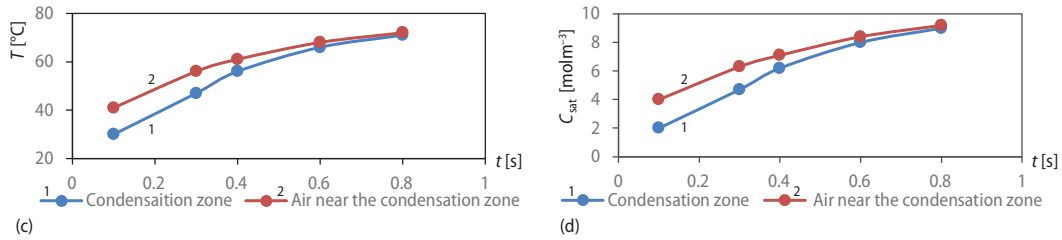
Figure 6. Temperature (c) and concentration (d) variations as function of time: T_h = 80 °C, T_0 = 22 °C, H = 50\% and \theta_0 = 80^\circ
