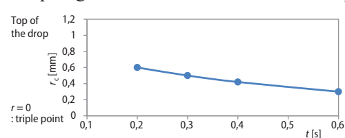
Figure 12. Evolution of the position of the transition point c at interface liquid-gas (from triple point to top of drop) as function of time: T_h = 70 \text{ }^\circ\text{C} , T_0 = 22 \text{ }^\circ\text{C} , H = 40\% and \theta_0 = 65^\circ
