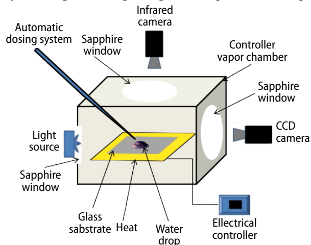
Figure 9. Schema of the experimental set-up
