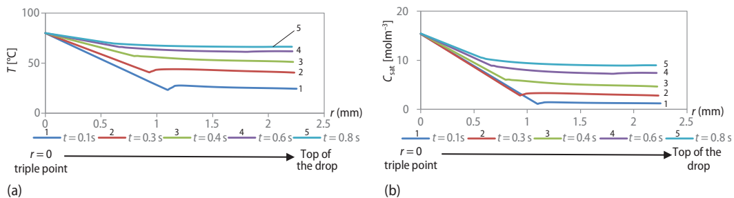
Figure 4. Temperature (a) and concentration (b) variations at liquid-gas interface (from triple point to top of drop) for different times: T_h = 80\text{ }^\circ\text{C} , T_0 = 22\text{ }^\circ\text{C} , H = 50\% and \theta_0 = 80^\circ
