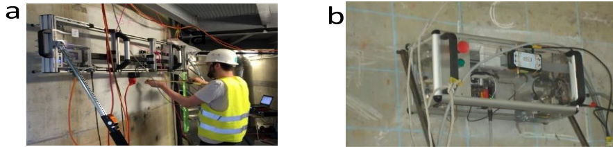
FIGURE 1. (a) The LWSF scanner during leakage test in VeRCoRs mock up . (b) The HFSW scanner during leakage test in VeRCoRs mock up.
