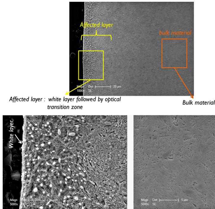
Fig. 2. Sub-surface microstructure relative to specimen 4.
