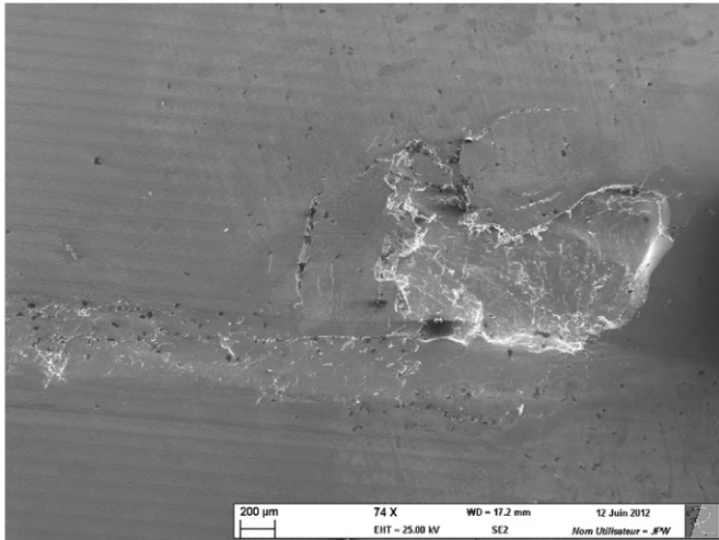
Fig. 9. SEM image of a spall formed on the surface of precision hard turned specimen 1.
