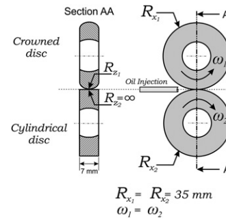
Fig. 8. Geometry of rolling contact fatigue test specimen.
