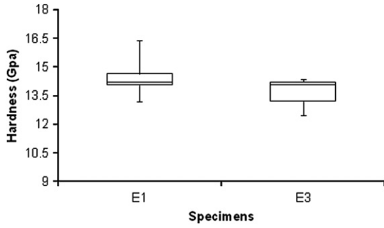
Fig. 5. Surface nanohardness (200 nm penetration depth).
