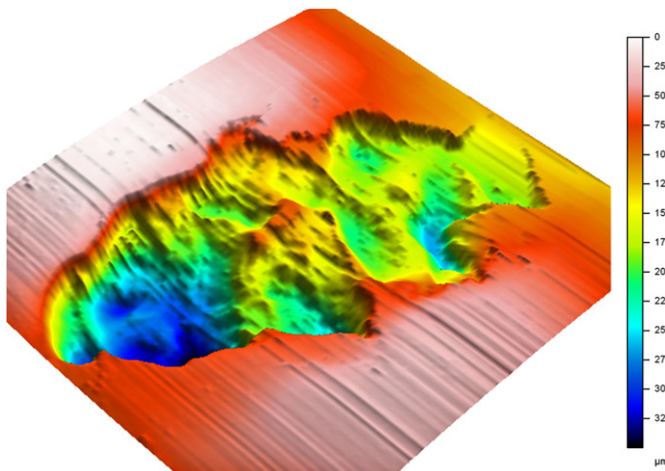
Fig. 10. 3D image of surface spall.
