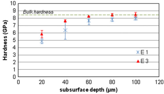
Fig. 6. Sub-surface nanohardness.
