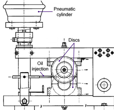
Fig. 7. Schematic view of twin-disc test rig.
