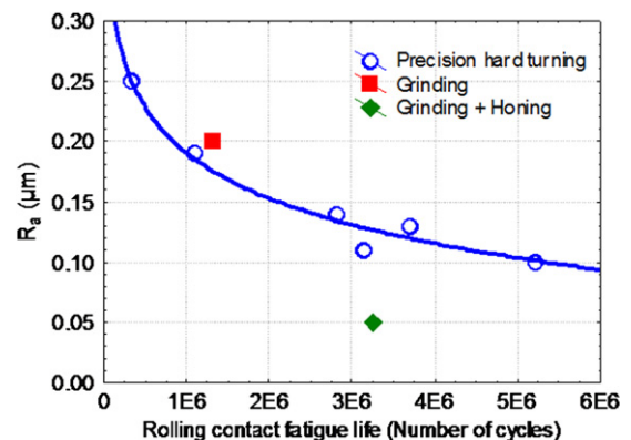
Fig. 12. Life comparison of precision hard turned vs. ground, and ground followed by honed specimen.
