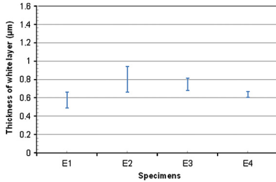
Fig. 3. Thickness evolution of the white layer.
