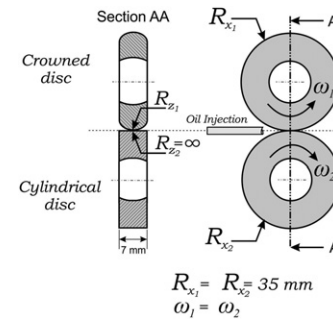
Fig. 8. Geometry of rolling contact fatigue test specimen.
