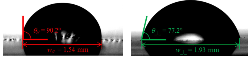
Figure 7. Example of anisotropy influence on apparent contact angle for parallel view (left) and perpendicular view (right) of a sessile drop (volume \sim 1\mu\text{L} ) deposited onto the SA8 sample.
