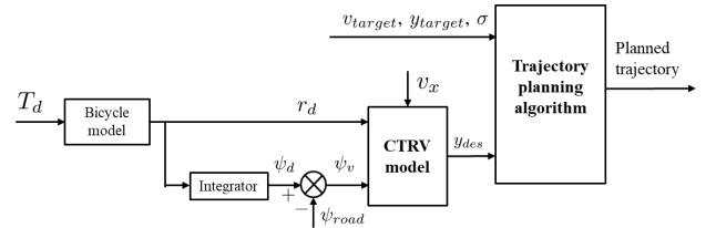
Fig. 4. Detailed view of the "Trajectory planning" module in Fig. 1.
