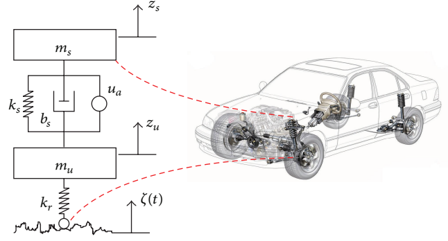
FIGURE 1: Active suspension system for a quarter wheel.
