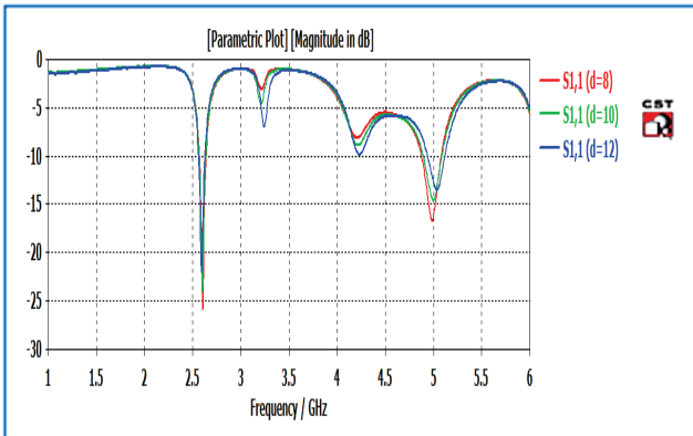
Fig. 9. Reflection coefficient for different values of d
