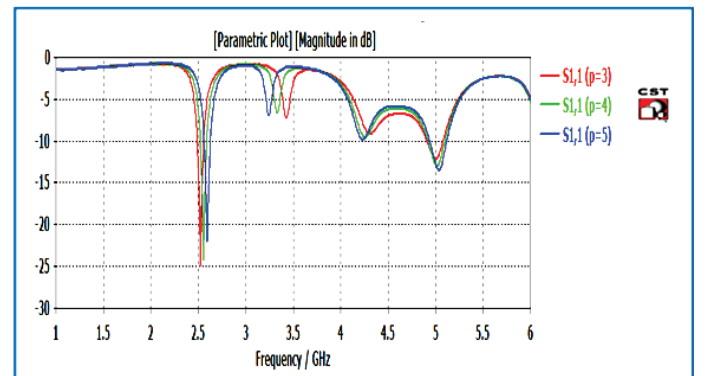
Fig. 8. The return loss of antenna with different values of p
