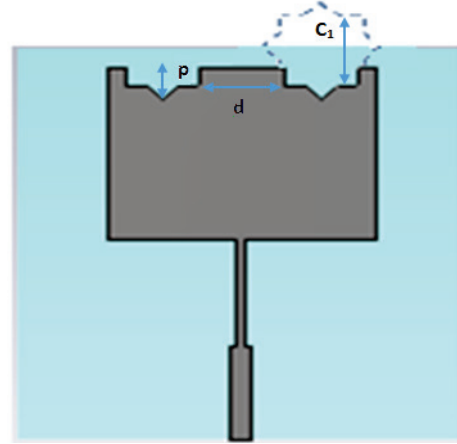
Fig. 7. Rectangular antenna with two star slots
