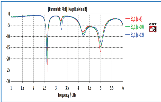
Fig. 9. Reflection coefficient for different values of d
