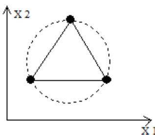
Fig. 4. Geometric representation of simplex
