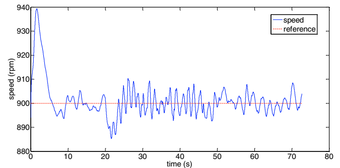
Fig. 6. Engine idle speed
