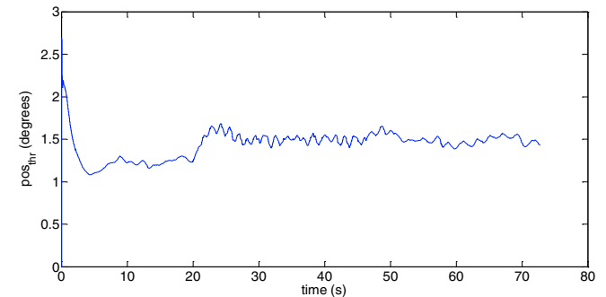
Fig. 7. Throttle command signal
