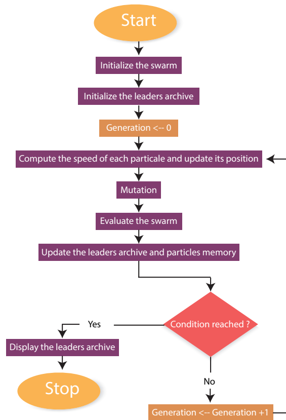
Figure 3: Flowchart of SMPSO algorithm
