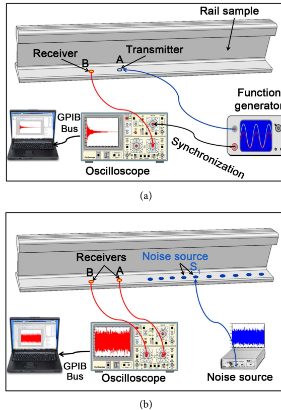
Figure 2. Experimental setup. (a) Active experiment; (b) Noise-correlation experiment.
