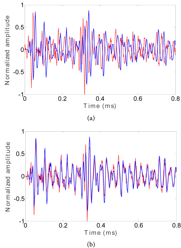
Figure 6. Comparison between the measured active response s_{AB}(t) (—) and \tilde{D}_{AB}^+(t) obtained from the estimated noise-correlation following Equation (3) for N = 10 noise sources (---). (a) Raw waveforms; (b) Waveforms with phase shift compensation.
