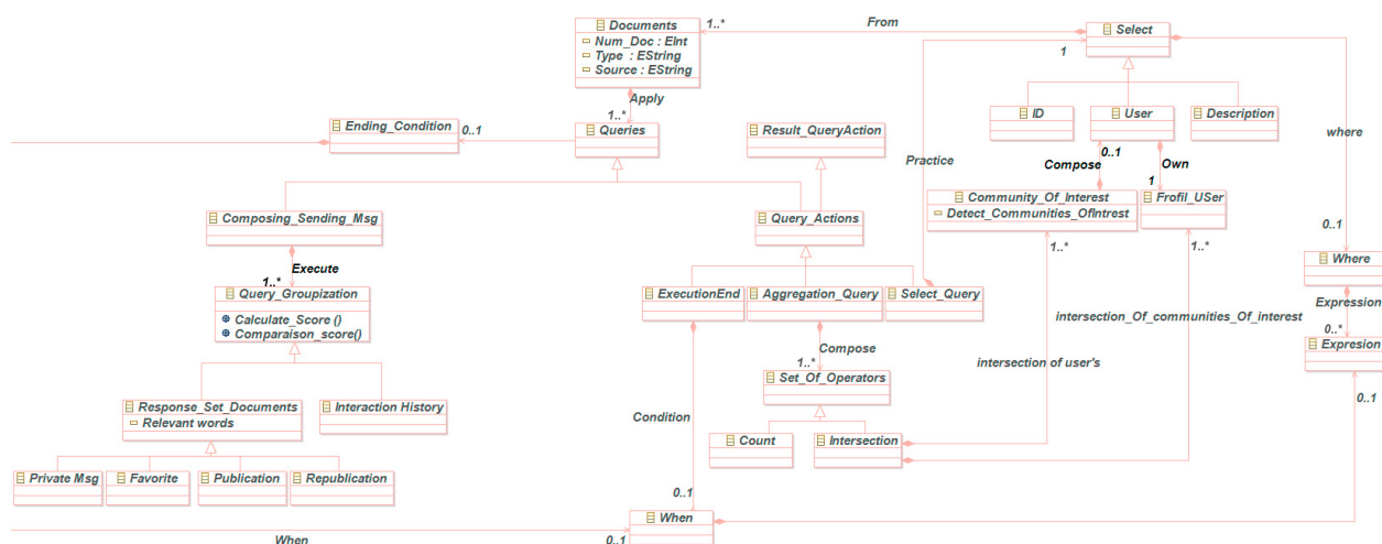
Fig. 4: An excerpt of the second DSL meta-model
