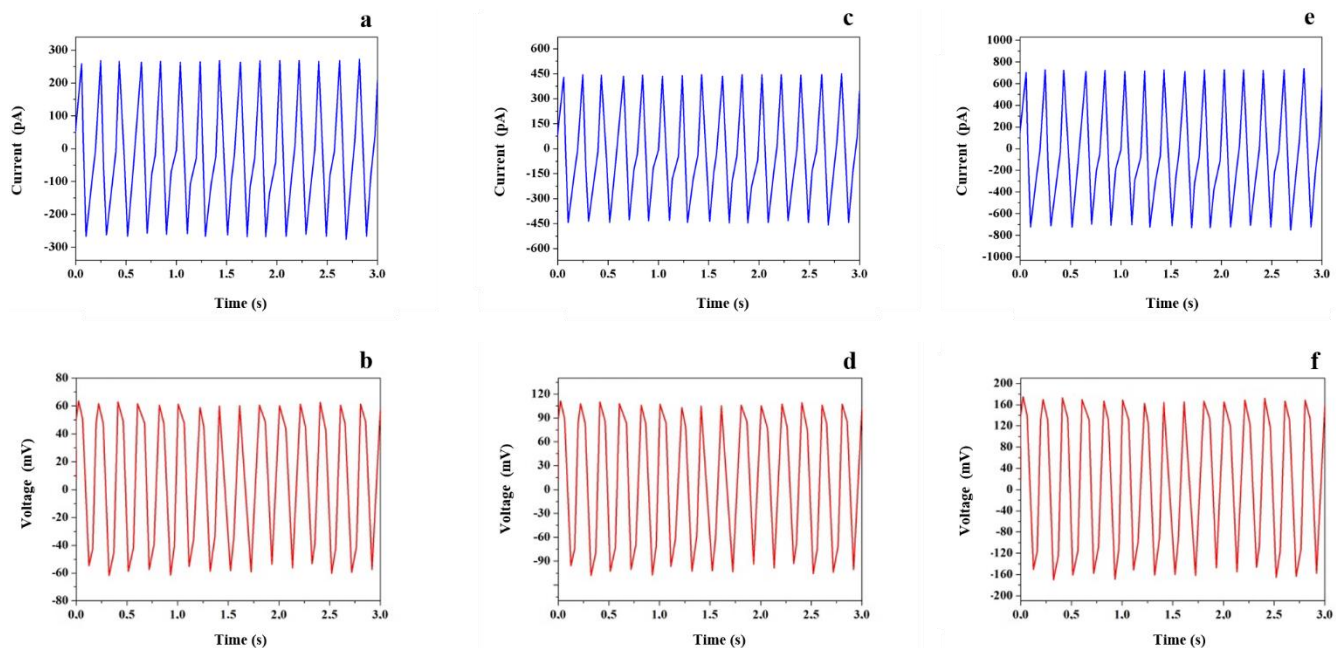
Figure 10. Electrical characteristics harvested by EVA 65% as a function of time under a transverse displacement with various values of strain S_M . (a) current harvested with S_M : 0.25%, (b) voltage harvested with S_M : 0.25%, (c) current harvested with S_M : 0.50%, (d) voltage harvested with S_M : 0.50%, (e) current harvested with S_M : 0.75%, (f) voltage harvested with S_M : 0.75%.
