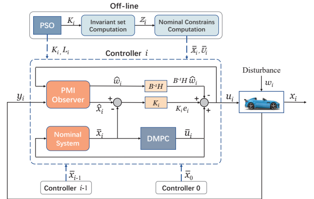
Fig. 3. Structure of the proposed integrated control scheme.
