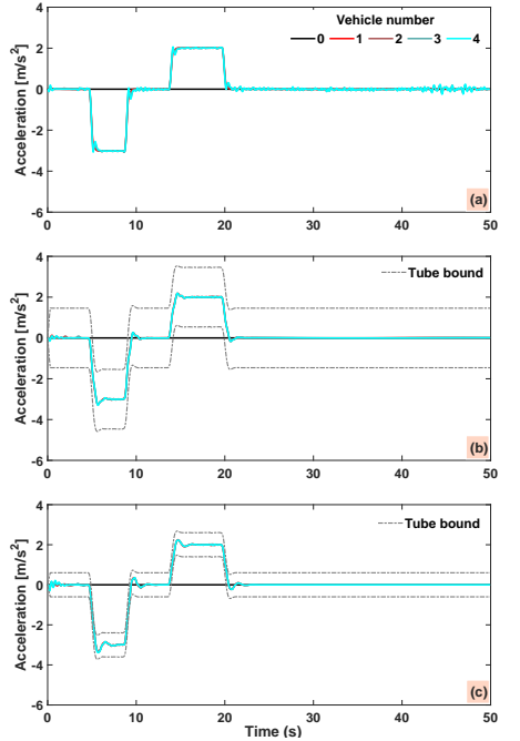
Fig. 13. Acceleration of following vehicles. (a) Classical DMPC, (b) RN MPC in [30], (c) Proposed controller.
