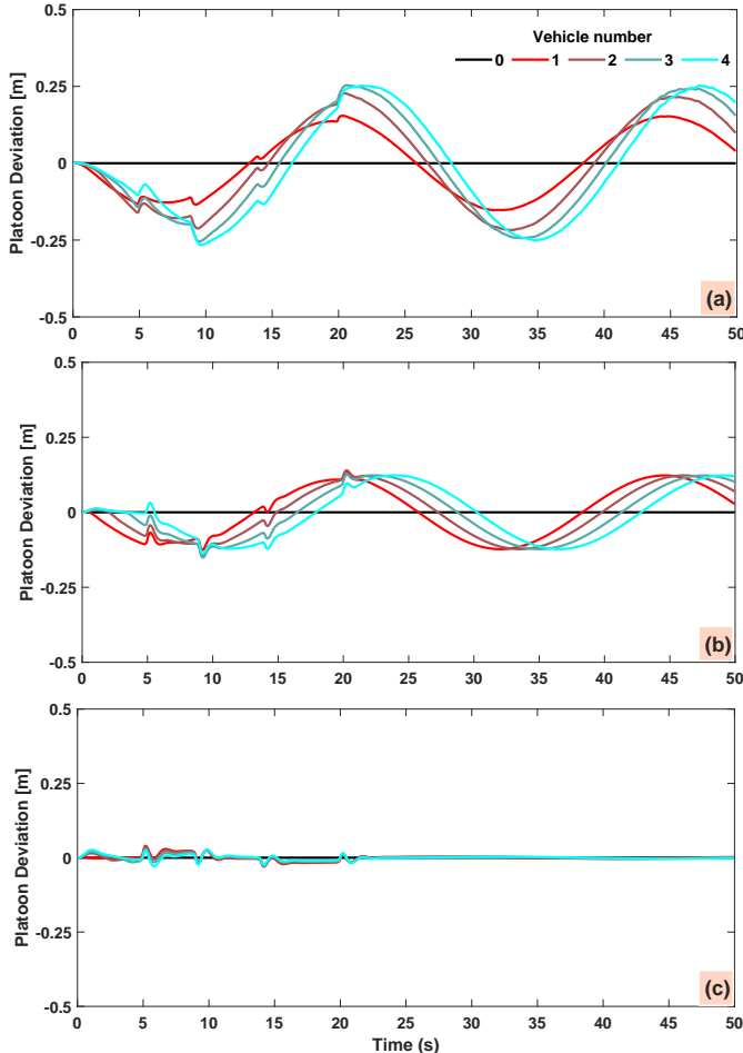
Fig. 10. Platoon deviation \Delta d_p . (a) Classical DMPC, (b) RNMPc in [30], (c) Proposed controller.
