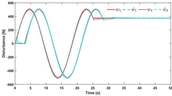
Fig. 8. Estimation of the lumped disturbance.
