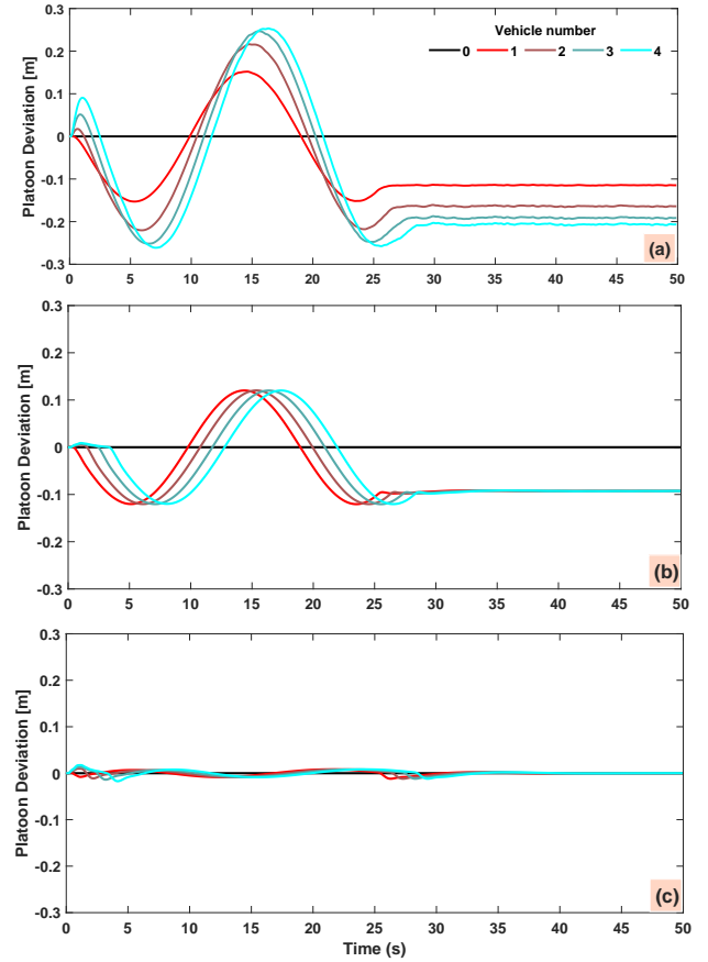
Fig. 4. Platoon deviation \Delta d_p . (a) Classical DMPC, (b) RN MPC in [30], (c) Proposed controller.
