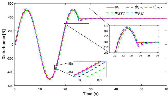
Fig. 9. Estimation of the lumped disturbance with different types of observers.
