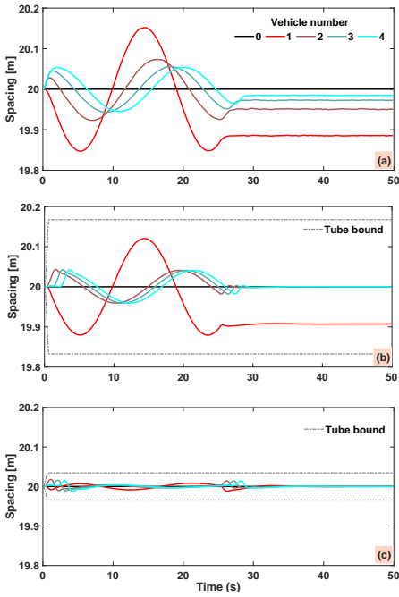
Fig. 5. Adjacent spacing d_s . (a) Classical DMPC, (b) RN MPC in [30], (c) Proposed controller.
