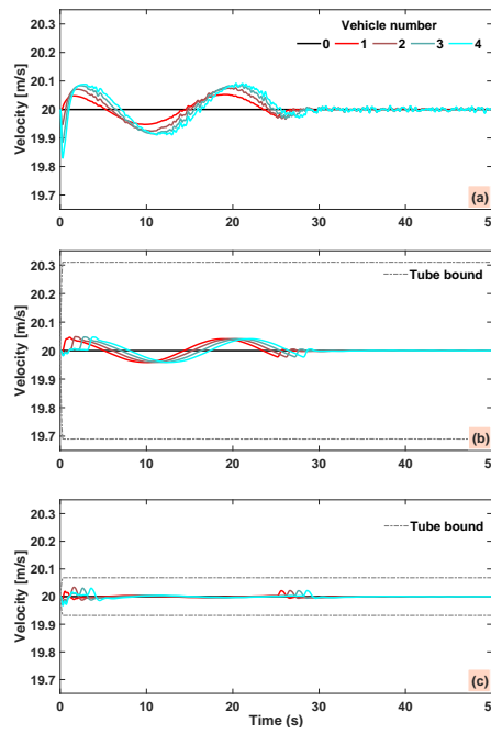
Fig. 6. Velocity of following vehicles. (a) Classical DMPC, (b) RN MPC in [30], (c) Proposed controller.
