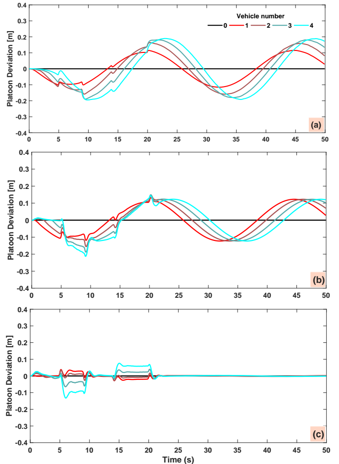
Fig. 15. Platoon deviation \Delta d_p (with PF communication topology). (a) Classical DMPC, (b) RN MPC in [30], (c) Proposed controller.
