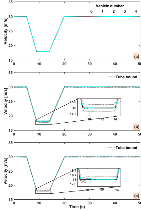
Fig. 12. Velocity of following vehicles. (a) Classical DMPC, (b) RN MPC in [30], (c) Proposed controller.
