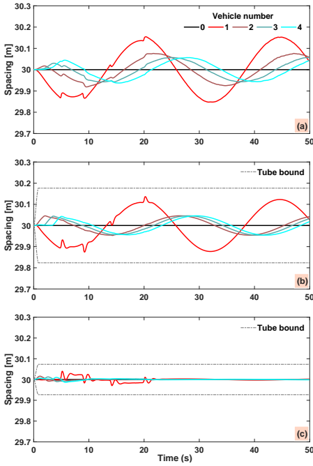
Fig. 11. Adjacent spacing d_s . (a) Classical DMPC, (b) RN MPC in [30], (c) Proposed controller.
