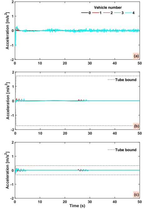
Fig. 7. Acceleration of following vehicles. (a) Classical DMPC, (b) RN MPC in [30], (c) Proposed controller.
