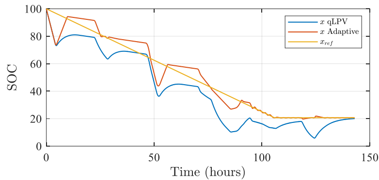
Fig. 7: SOC profiles comparison (simulation result).
