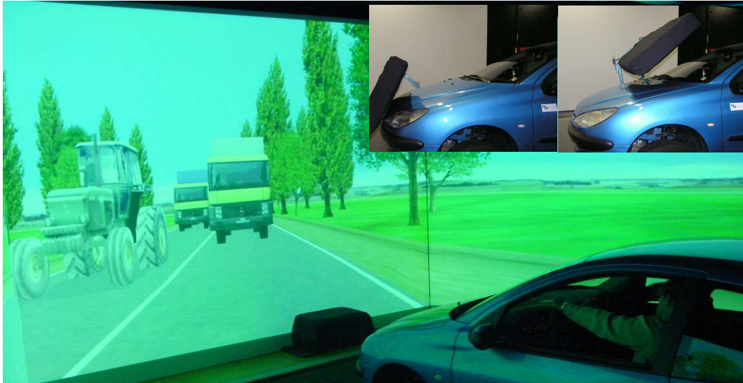
Figure 2 Scenario of the unavoidable crash situation; Sequence of the falling block on the windscreen
