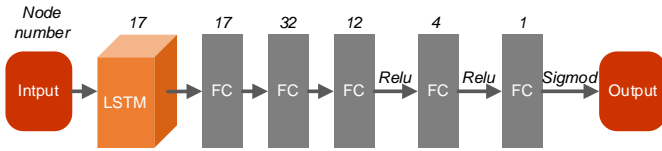
Fig. 2. Network structure of the LSTM method in lane change intention prediction.
