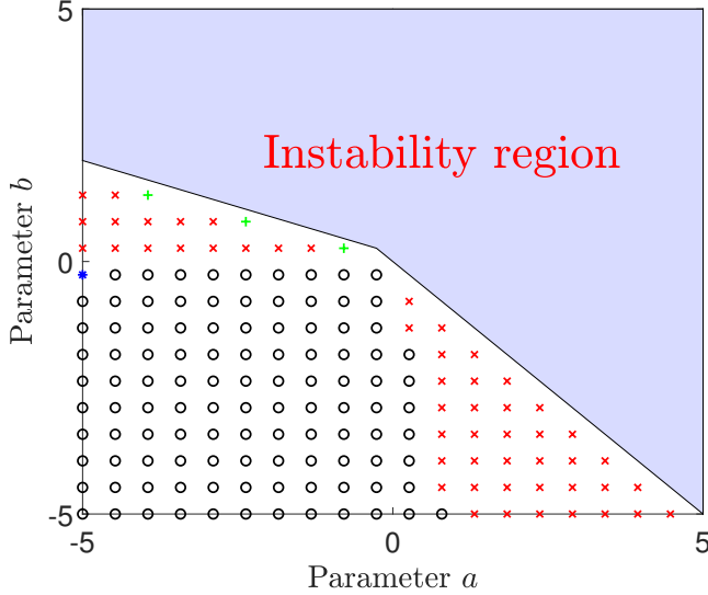
Fig. 6: Feasibility regions obtained with [41, Theorem 4.3] (o), [42, adapted Theorem 5] (o,*), adapted Theorem 1 with a quadratic Lyapunov function (o*,*), Theorem 1 (o*,*,+).
