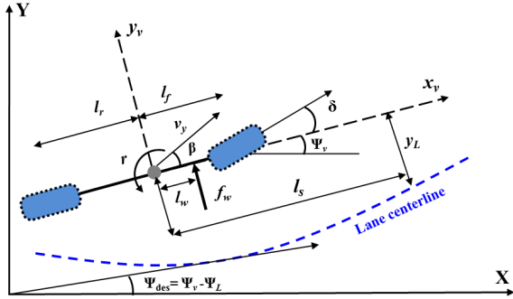
Figure 1: Schematic of a two degrees-of-freedom vehicle model.
