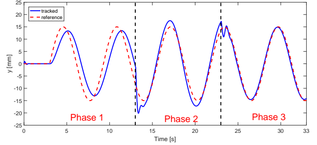
Fig. 10. Three-phase fast trajectory tracking along the y -axis in Scenario 2.
