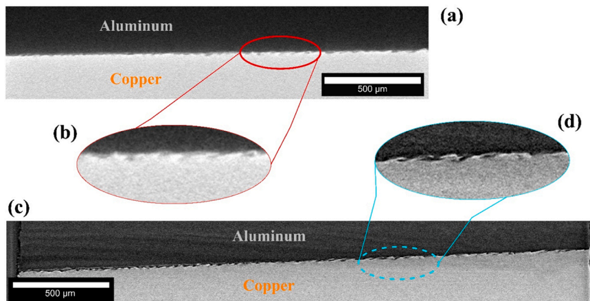
Fig. 2. Comparison of a tomographic section for an Al/Cu interface MPW joint, (a) – Laboratory X-ray absorption tomographic section, (b) – Close-up of the interface for the laboratory source, (c) – Synchrotron propagation-based phase contrast section, (d) – Close-up of the interface for the synchrotron source.
