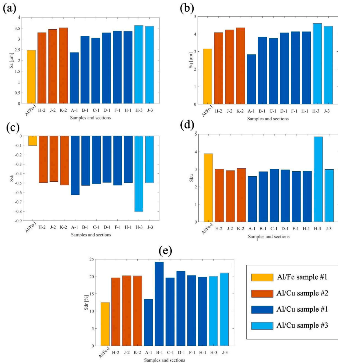
Fig. 6. Topographic roughness parameters analysis on the surfaces extracted from the interfaces – (a) Sa parameter, - (b) Sq parameter, - (c) Ssk parameter, - (d) Sku parameter, - (e) Sdr parameter.
