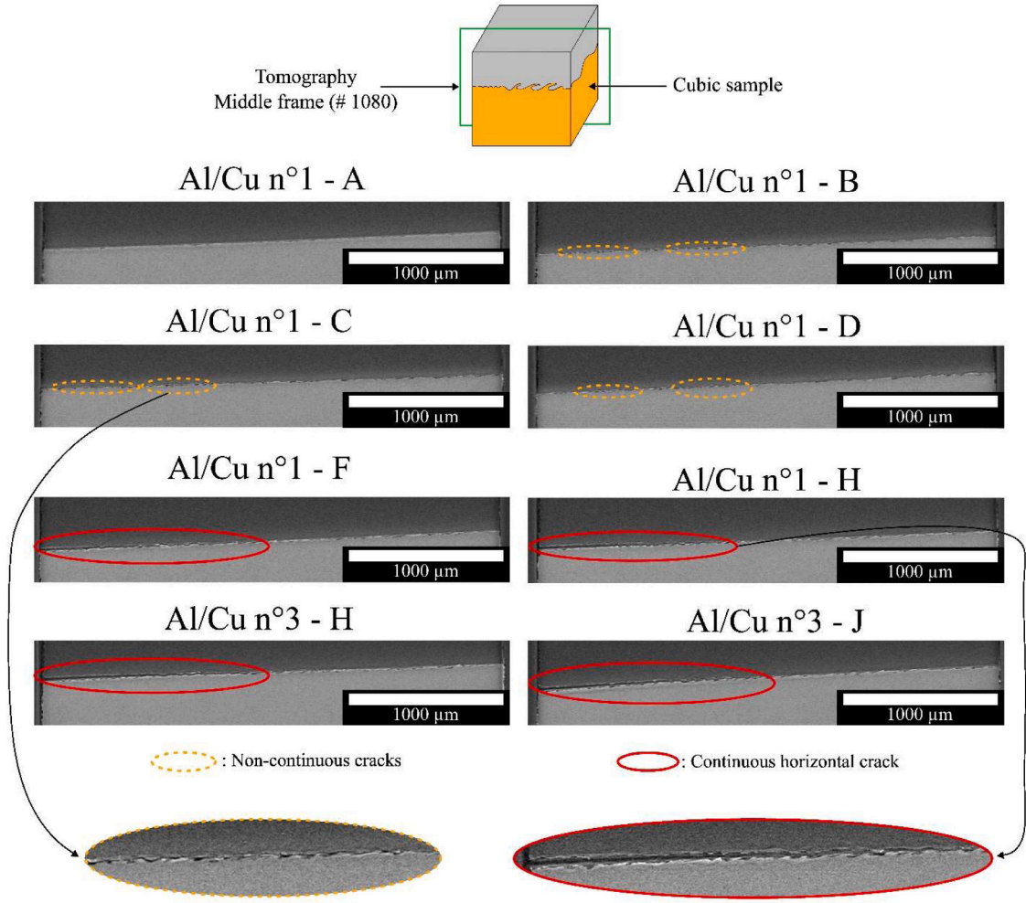
Fig. 10. Cracks comparison at the center of the cubes (frames #1080) – Plan (XZ).
