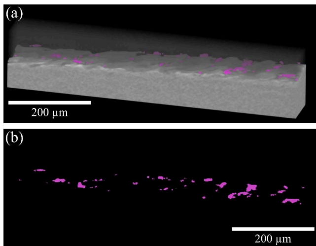
Fig. 8. Porosities and cavities localization from the Al/Cu cross-section presented in Fig. 7 – voxel size 1.28 \mu\text{m} , (a) – View with copper, aluminum and porosities (pink), (b) – View with porosities only.
