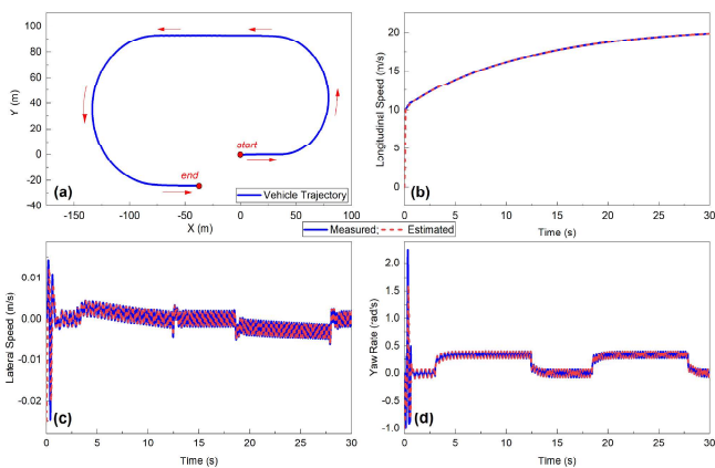
Fig. 8. Estimation performance in Scenario 3. (a) Vehicle trajectory. (b) Longitudinal speed v_x . (c) Lateral speed v_y . (d) Yaw rate r .
