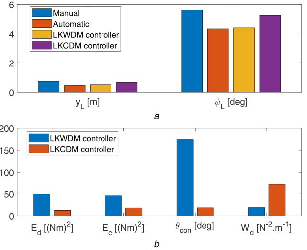
Fig. 9 Performance evaluation
