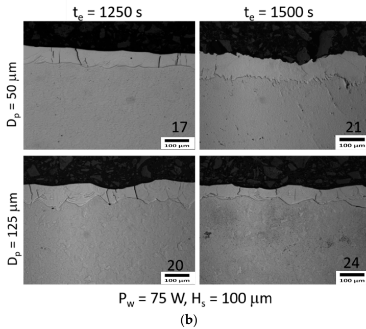
Figure 8. Images of the cross-section of coatings obtained by optical microscopy. The number (a) for H_s = 50 \mu\text{m} and d_p = 50 \mu\text{m} (b) P_w = 75 \text{ W} and H_s = 100 \mu\text{m} .
