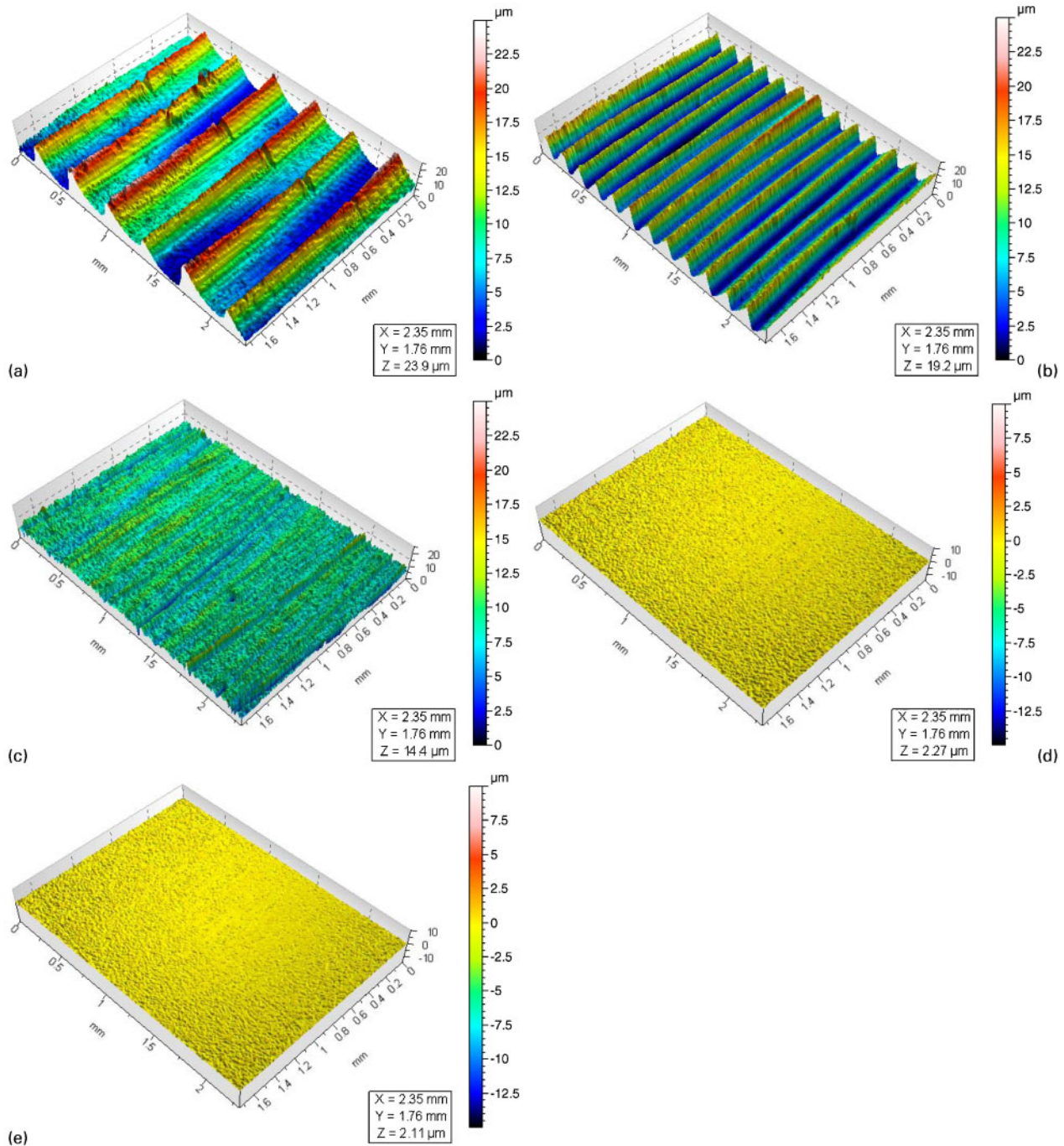
2 Morphologies of rough surfaces prepared on plane specimens by a, b milling and c-e wet grinding processes: a surf. 1; b surf. 2; c surf. 3; d surf. 4; e surf. 5
