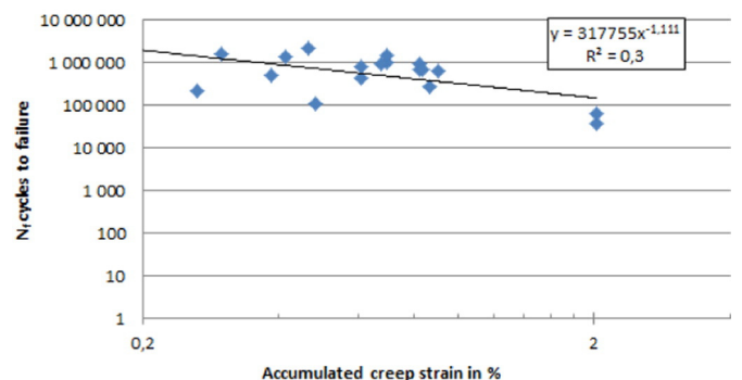
Fig. 16. N_f cycles to failure in function of the accumulated creep strain in the top solder.
