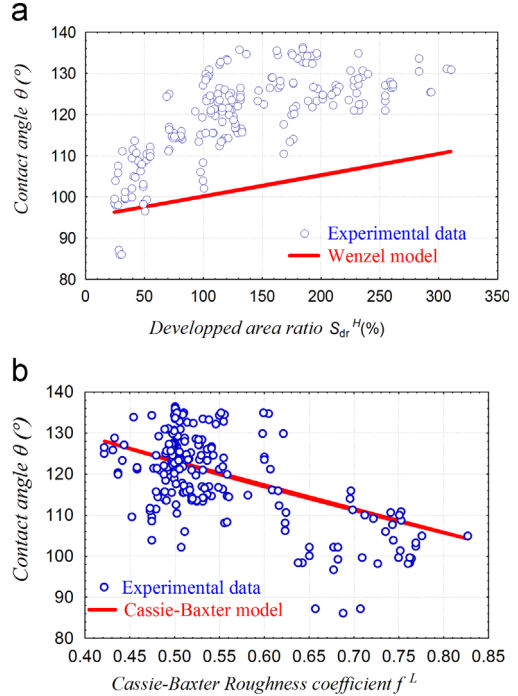
Fig. 9. Contact angle versus roughness parameters calculated at their relevant scale (a) Comparison of the Wenzel model, \cos \theta=r^H * \cos (\theta_0) , and the experimental data. (b) Comparison of the Cassie–Baxter model, \cos \theta=f^L \cos (\theta_0)-(1-f^L) , and experimental data, where f^L=S_{ha}/(S_{ha}+S_{da}) , r^H=(S_{dr}+100)/100 , and \theta_0 is the contact angle on a flat surface of the polymer.
