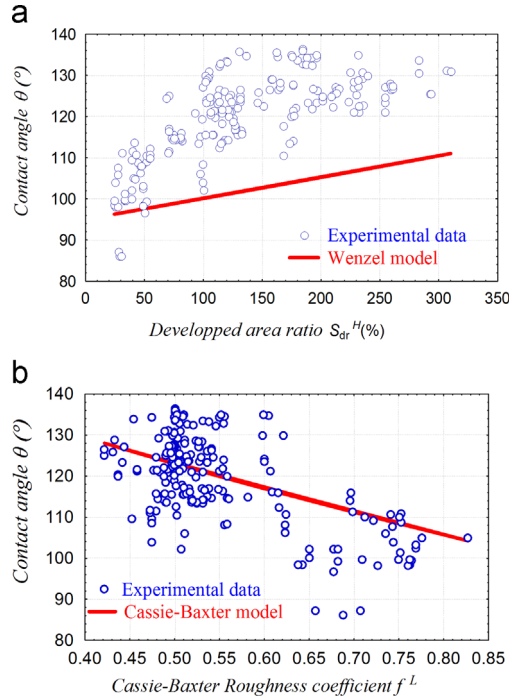
Fig. 9. Contact angle versus roughness parameters calculated at their relevant scale (a) Comparison of the Wenzel model, \cos \theta = r^H \cos(\theta_0) , and the experimental data. (b) Comparison of the Cassie–Baxter model, \cos \theta = f^L \cos(\theta_0) - (1-f^L) , and experimental data, where f^L=S_{ha}/(S_{ha}+S_{da}) , r^H=(S_{dr}+100)/100 , and \theta_0 is the contact angle on a flat surface of the polymer.
