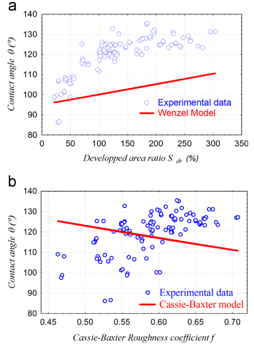
Fig. 8. Contact angle versus roughness parameters calculated at the whole scale (a) Comparison of the Wenzel model, \cos \theta = r^H \cos(\theta_0) , and experimental data. (b) Comparison of the Cassie–Baxter model, \cos \theta = f^L \cos(\theta_0) - (1-f^L) , and experimental data, where f^L=S_{ha}/(S_{ha}+S_{da}) , r^H=(S_{dr}+100)/100 , and \theta_0 is the contact angle on a flat surface of the polymer.
