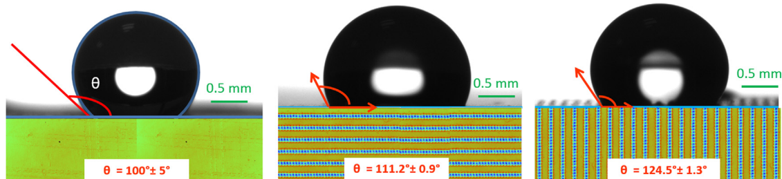
Fig. 3. Representation of the experimental measurements of the contact angle on a smooth surface and a textured surface in both directions of the surface texture.
