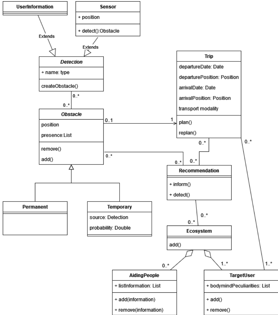
Fig. 4. UML classes diagram to model notions and the relations between them to provide the support system.
