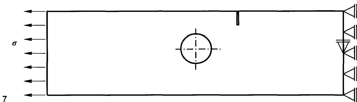
Fig. 69: Boundary conditions applied on the perforated SEN specimen
