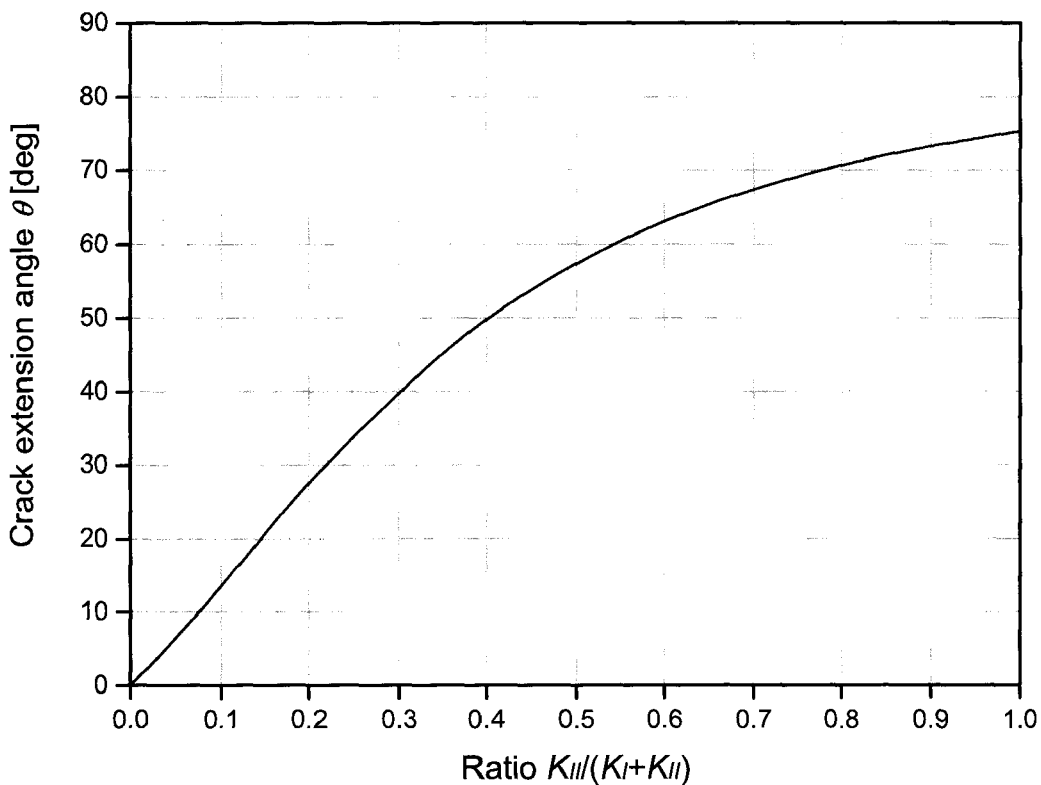
Fig. 27: MERR criterion - crack propagation angle \theta = f(K_{II}/(K_I + K_{II}))
