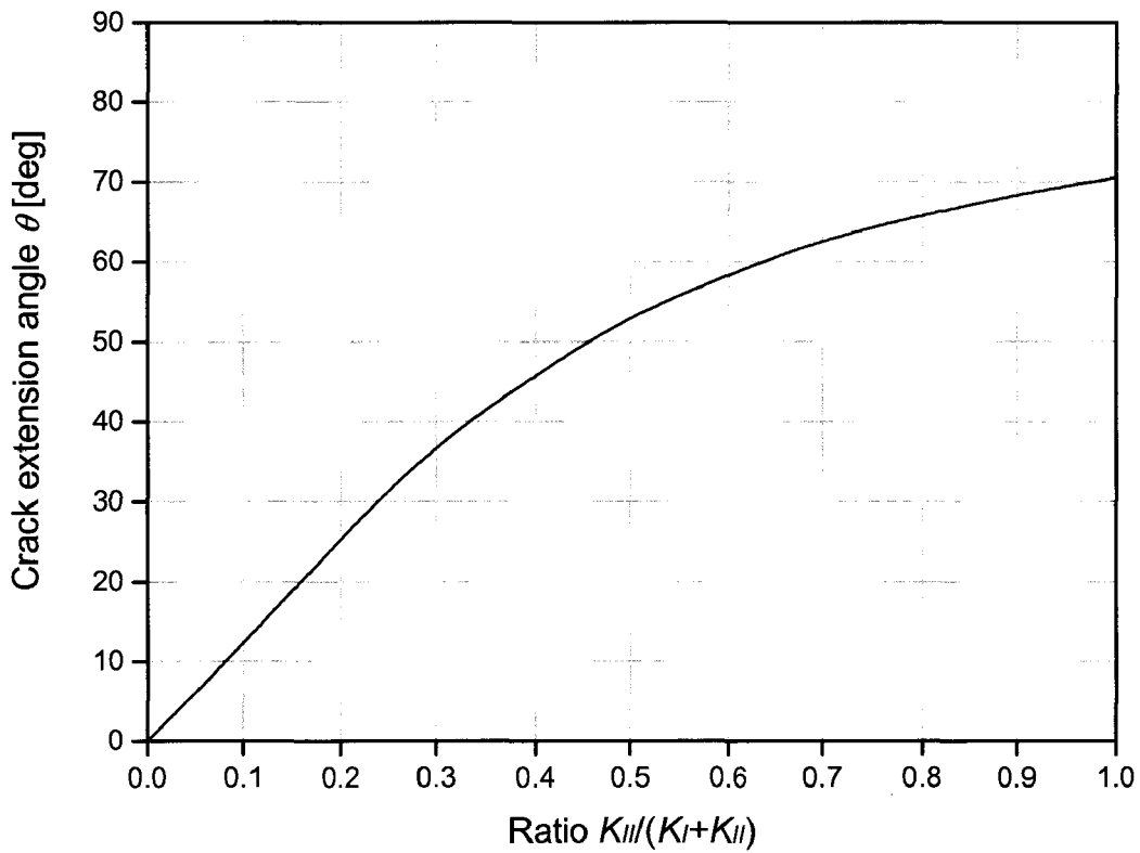
Fig. 25: MTS criterion - crack propagation angle \theta = f(K_{II}/(K_I + K_{II}))
