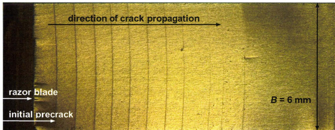
Fig. 122: Crack front geometry after successive load-unload cycles for unfilled Mat1 at ambient temperature
