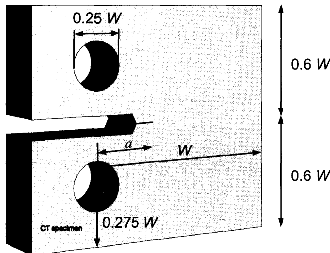
Fig. 59: Compact Tension specimen dimensions
