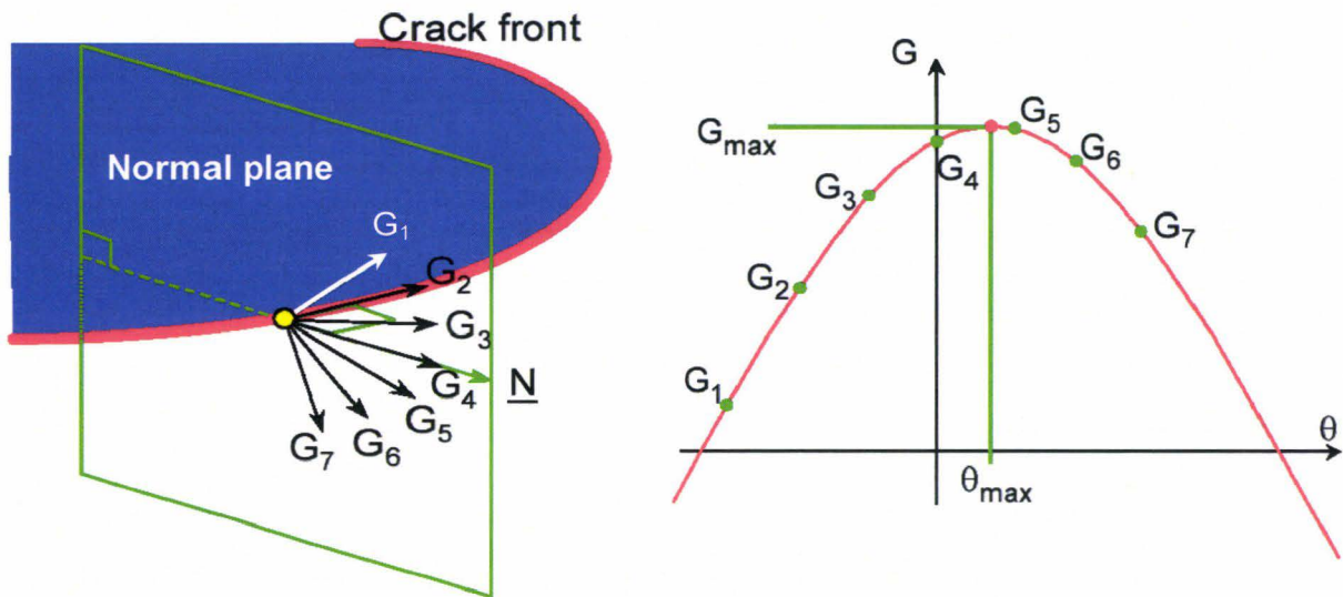
Fig. 48: Energy based calculation of G_{max} and growth direction [Zen06]
