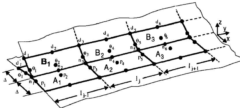
Fig. 44: VCCT - 27-noded brick element model [JiM03]
