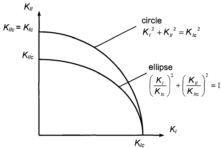
Fig. 32: Mixed-mode loading - Empirical fracture criteria
