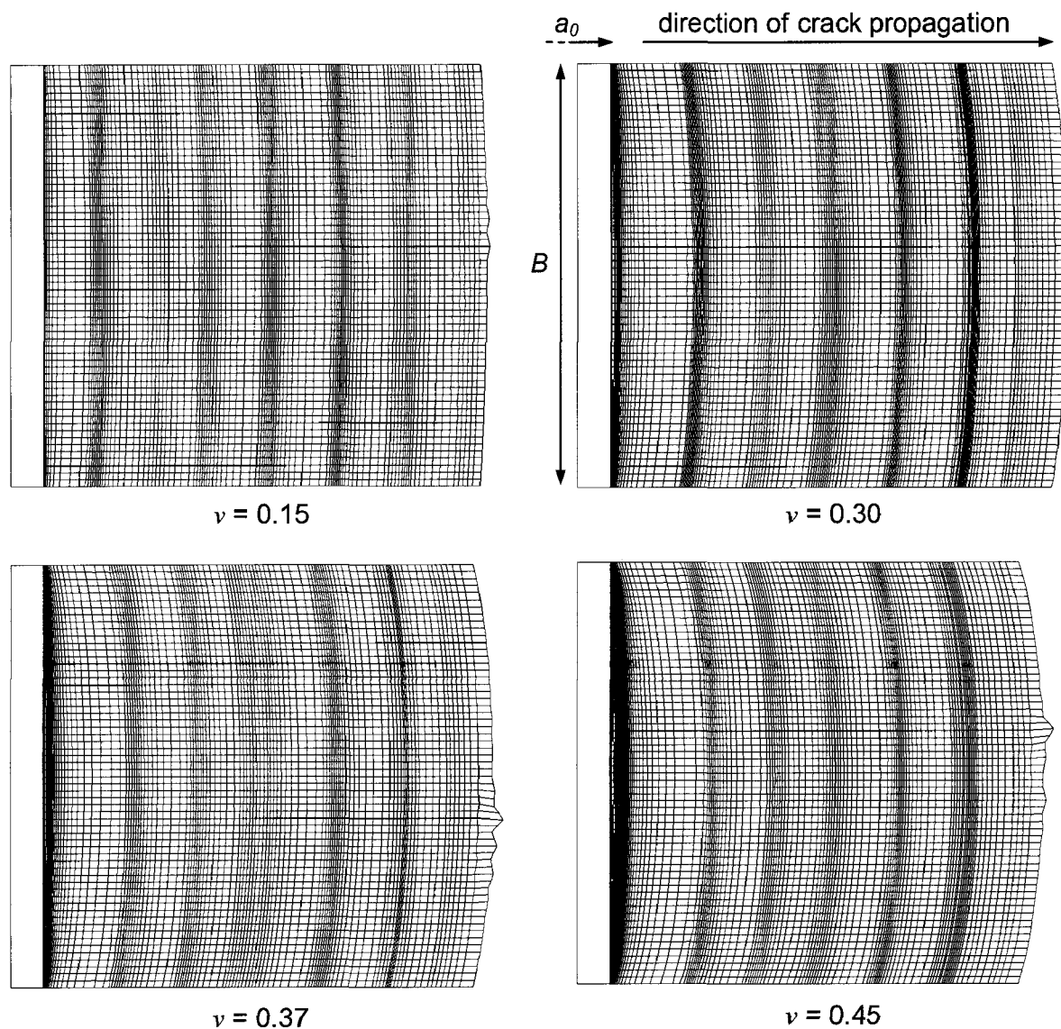
Fig. 73: Influence of the Poisson's ratio on numerical crack front curvature (fatigue crack propagation using a 3D model with an initial straight crack front and without plain strain boundary conditions)
