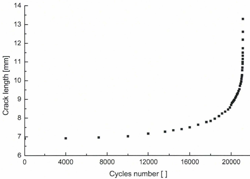
Fig. 113: Measured crack length
