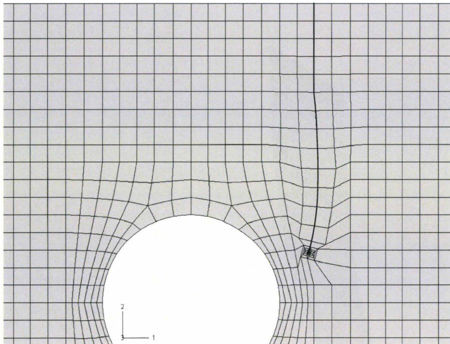
Fig. 85: Zencrack - Crack path obtained without relaxation (fine mesh)
