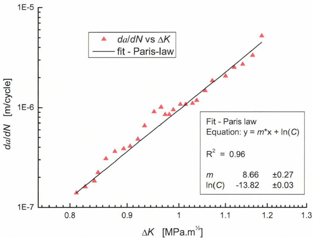
Fig. 116: Fitting of experimental data with a Paris law (evaluation of \Delta K based on Eq. 142 [A-647])
