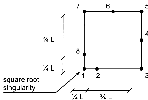
Fig. 35: 8-noded quarter point element
