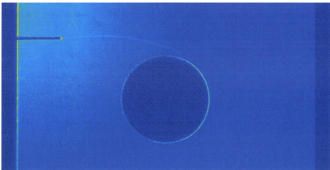
Fig. 111: Experimental crack path ( L = 7 mm)
