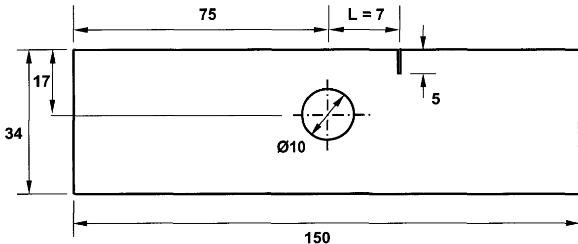
Fig. 68: Geometry of the perforated SEN specimen (dimensions in mm)
