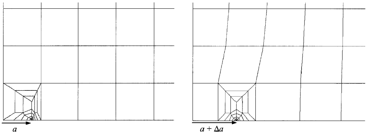
Fig. 58: Zencrack - Crack-block transfer [Zen06]
