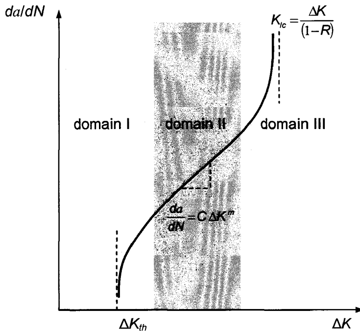
Fig. 65: Cyclic loading - Crack growth rate da/dN as a function of stress intensity factor range \Delta K
