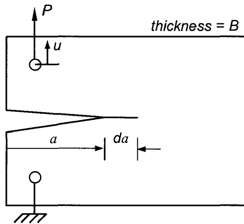
Fig. 7: Cracked plate subjected to an external load P
