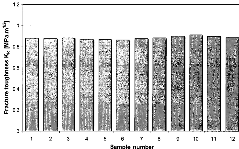
Fig. 93: K_{Ic} measurement for unfilled Mat1 (evaluation of K_{Ic} based on Eq. 138 [A-399])
