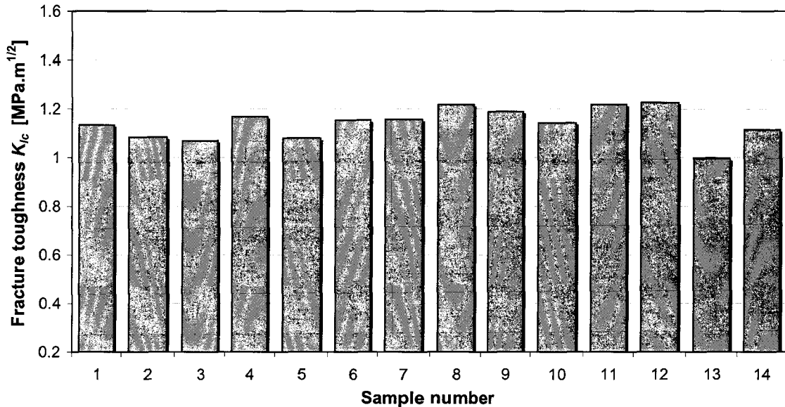
Fig. 90: K_{Ic} measurement for Mat1 (ambient temperature) (evaluation of K_{Ic} based on Eq. 138 [A-399])
