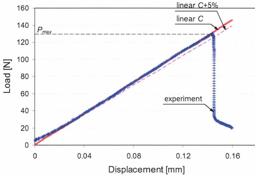
Fig. 60: Load-displacement curve (test realised with an epoxy resin material at T = 23°C)
