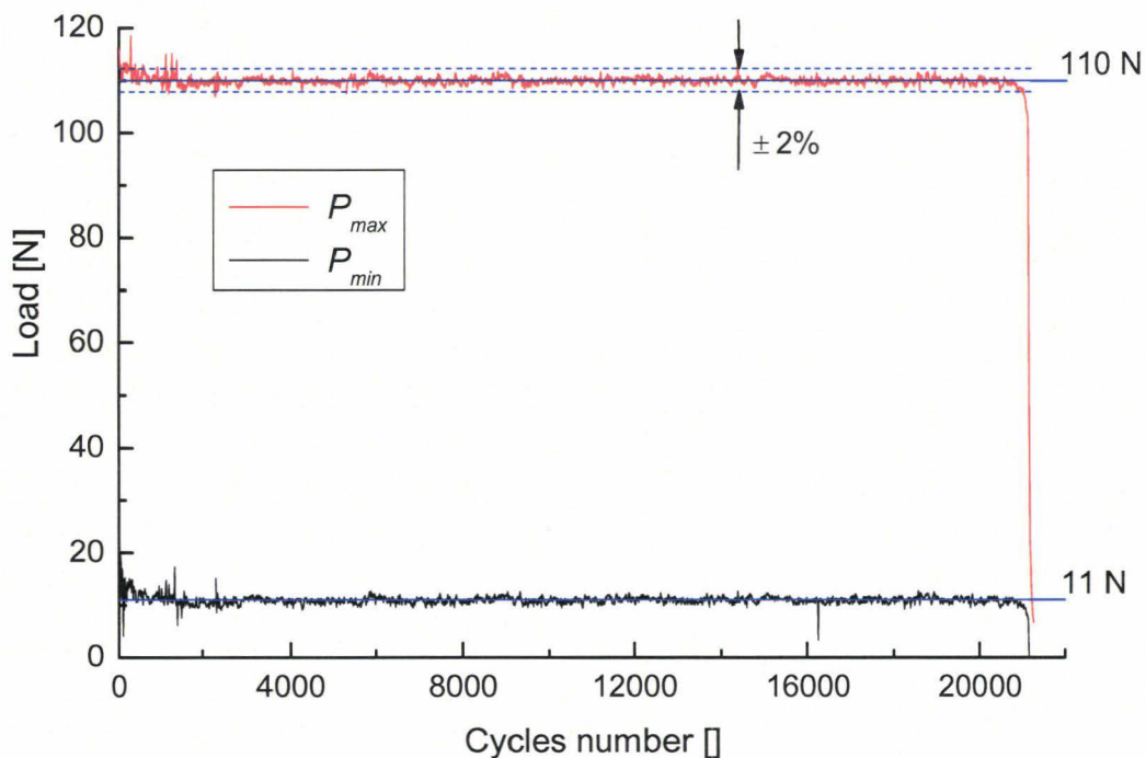
Fig. 114: Force applied and limits for valid data ( R = 0.1 , frequency 1 Hz)
