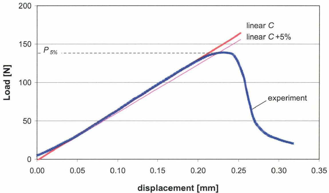
Fig. 98: Load-displacement curve for Mat2 at T = 130°C
