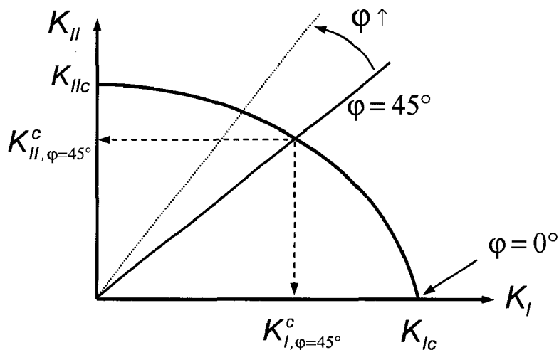
Fig. 108: Mixed-mode loading - Design of fracture criterion
