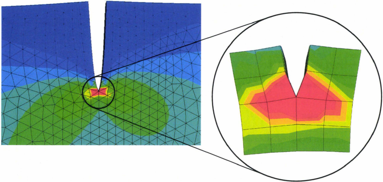
Fig. 53: Submodeling technique- Global model and associated submodel
