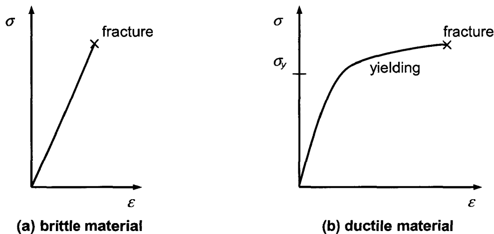
Fig. 2: Brittle and ductile material behaviour
