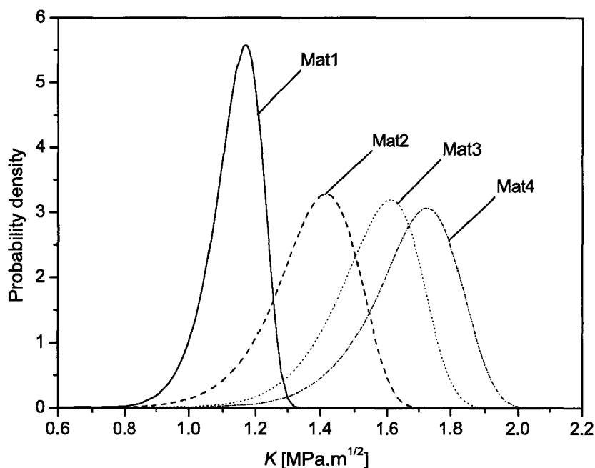
Fig. 96: Probability density function for Mat1-4
