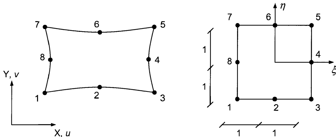
Fig. 34: 2D 8-noded isoparametric element
