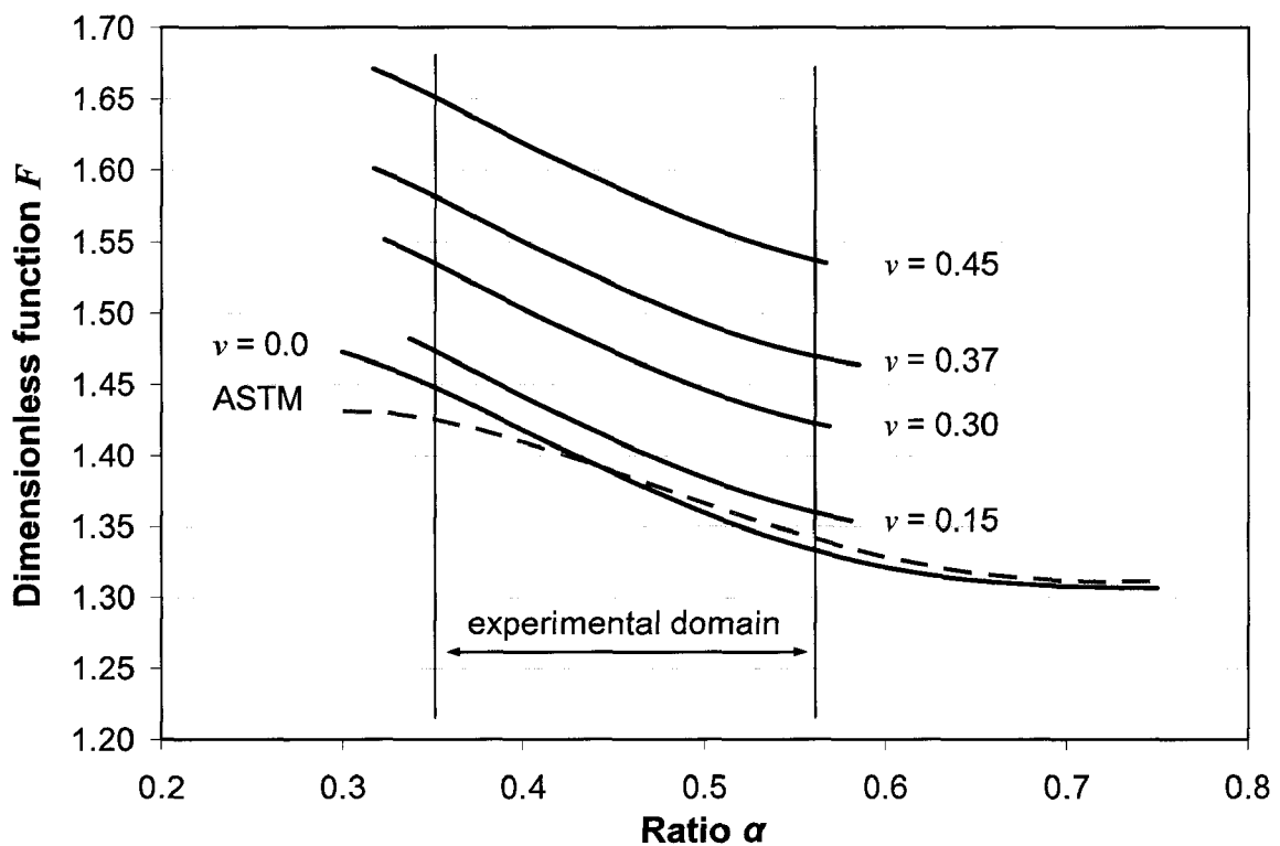
Fig. 76: Influence of Poisson's ratio on effective function F_{eff} (from FE models of CT specimen with B = 6 mm and W = 20 mm)
