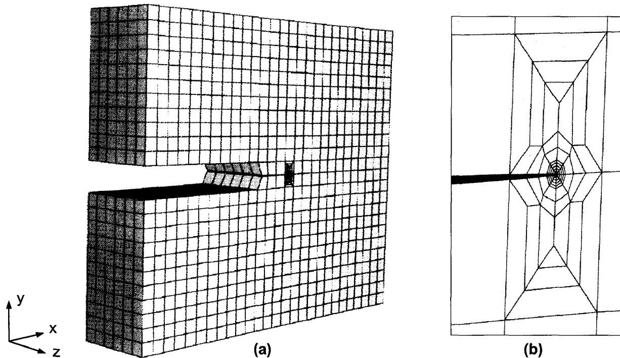
Fig. 70: (a) Numerical model of CT specimen; (b) crack-block at the crack tip
