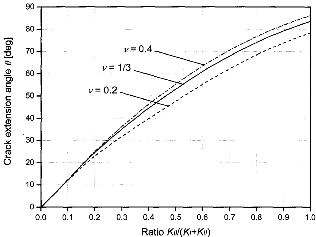
Fig. 28: MSED criterion - crack propagation angle \theta = f(K_{II}/(K_I + K_{II}))
