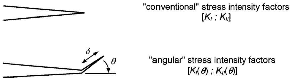
Fig. 26: Conventional and kinking fracture approach
