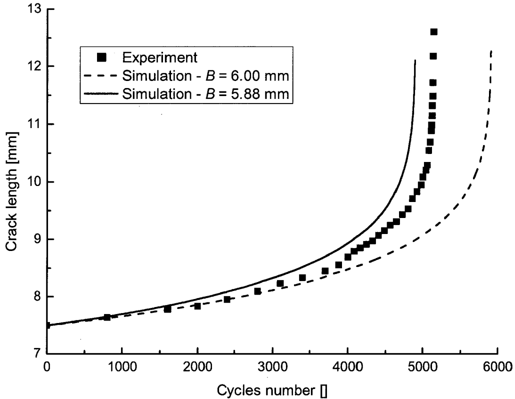
Fig. 121: Experimental and simulated crack length evolution (FE models with 2D plane strain assumption)
