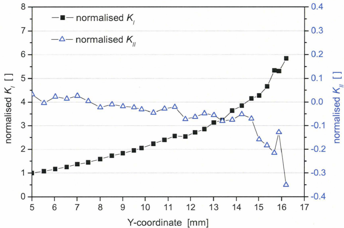
Fig. 83: ADAPCRACK3D - Normalised K_I and K_{II} as function of the Y-coordinate (normalised by K_I at the first increment)
