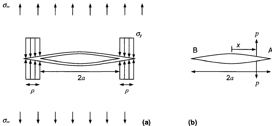
Fig. 21: a) Dugdale's plastic zone model b) Wedge forces
