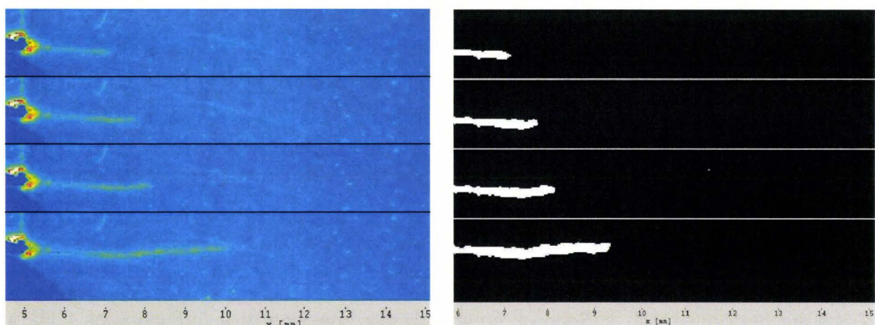
Fig. 63: Set of images recorded during a test and after post processing
