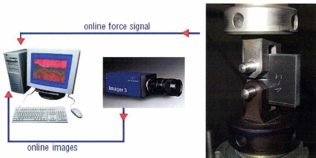
Fig. 62: Optical crack tracing (OCT) equipment
