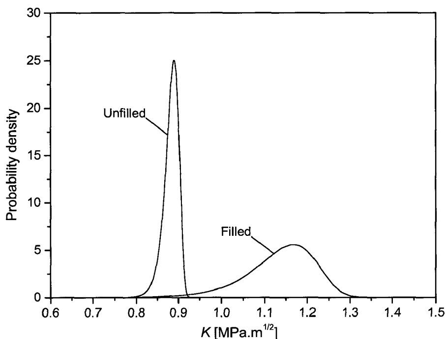
Fig. 95: Probability density function for filled and unfilled Mat1 at ambient temperature
