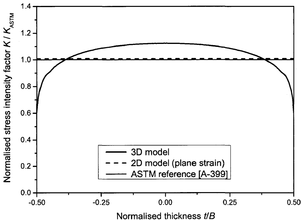
Fig. 72: SIF along the crack front for a FE model with a straight front profile
