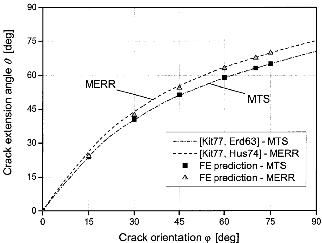
Fig. 77: CCT specimen - Prediction of the crack propagation direction
