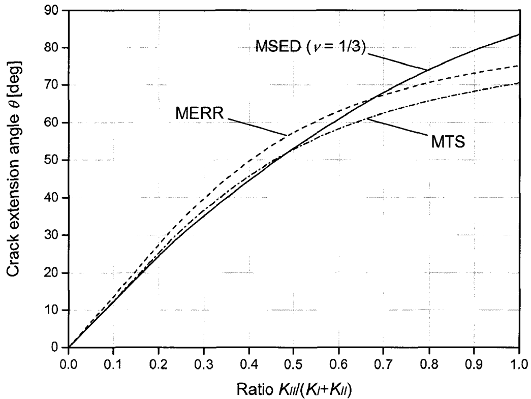
Fig. 29: Comparison between the MTS, MERR, and MSED criteria
