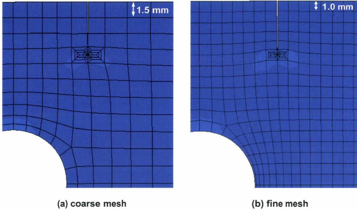
Fig. 84: Zencrack - Details of the coarse and fine FE models (initial crack length)
