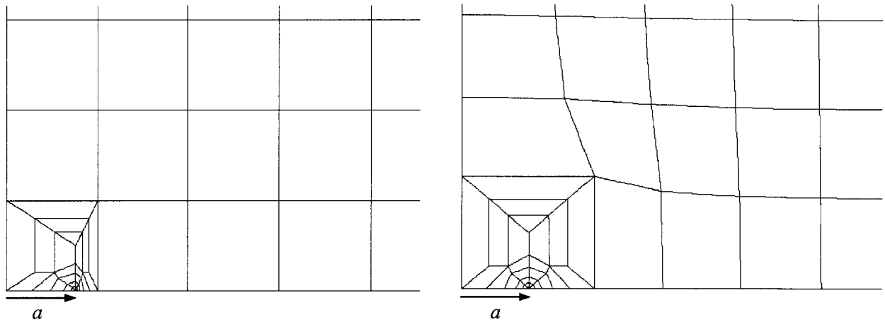
Fig. 57: Zencrack - Mesh relaxation [Zen06]
