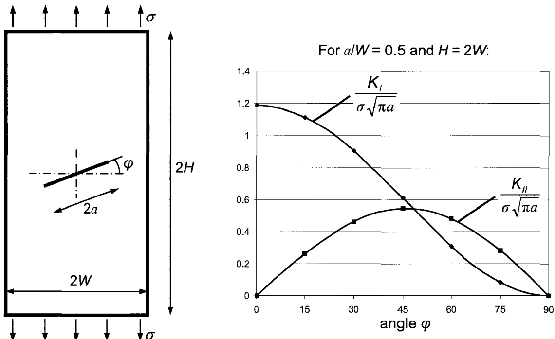
Fig. 67: Centre cracked tension CCT specimen [Wil71, Kit77, Mur87]
