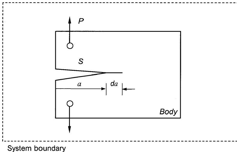
Fig. 6: Reversible thermodynamic system for energy balance concept [Gri21-24]
