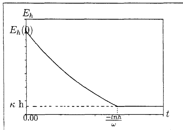
FIG. 5.1 – Behaviour of the right hand side of (5.45)
