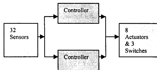
Fig. 2.11, RBD for 2-Cont Configuration
