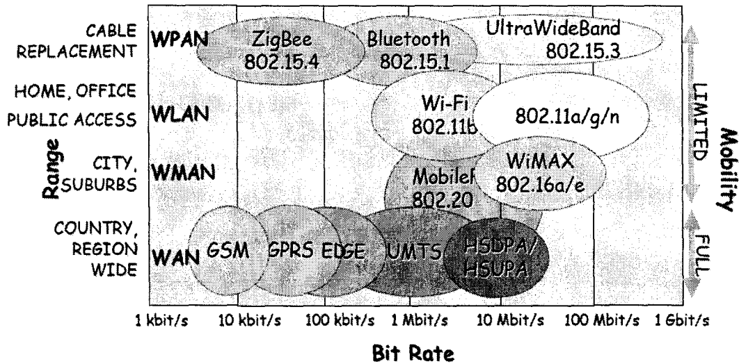
Fig. 3.1, Comparison of Different Technologies with Respect to Range, Bit Rate and Mobility [WTG]
