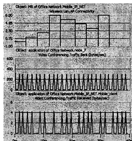
Fig. B, MN V=33Km/hr; IPT 90; MIPv4, Congested Model
