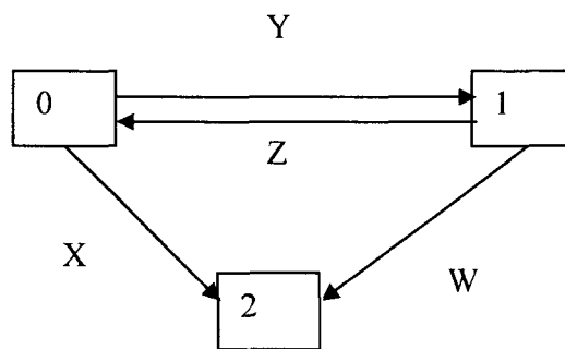
Fig. C. Markov Model
