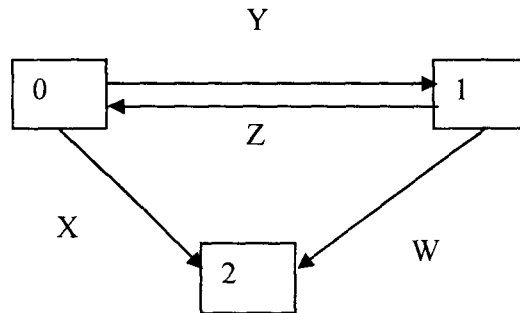
Fig. 2.8, Markov Model
