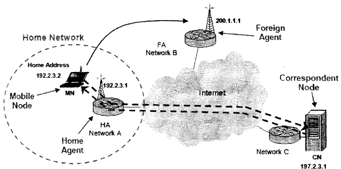
Fig. 3.6, IPv4 MN at HA [OPN]
