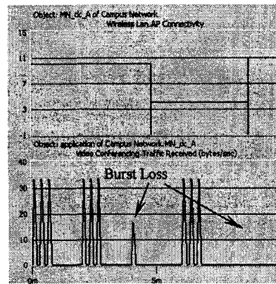
Fig. G, Complete Burst Loss in 3PB; t_{F2L}=36\text{sec}
