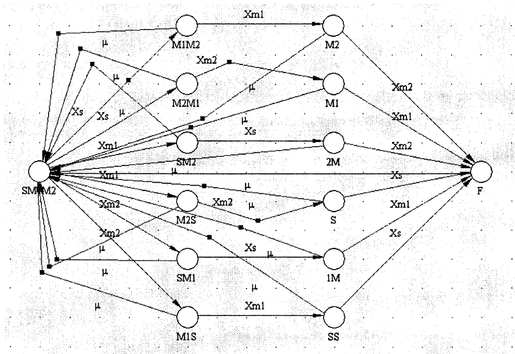
Fig. 2.10, Markov Model for Hierarchical NCS
