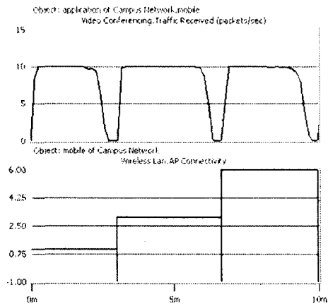
Fig. J, Traffic received in packets/second and AP connectivity for a mobile node moving at 33Km/hr in 802.11g architecture, transmit power 80mW
