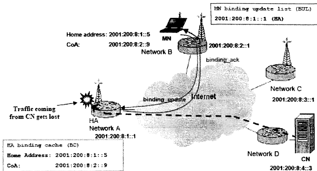
Fig.3.10, IPv6 MN Moves to Foreign Network [OPN]
