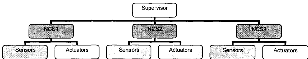
Fig. 2.5, Hierarchical Fault-Tolerant Controllers
