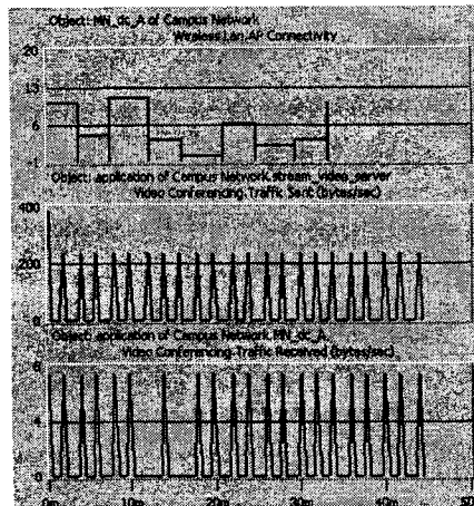
Fig. E, MN V=33Km/hr; IPT120; MIPv6, Congested Model
