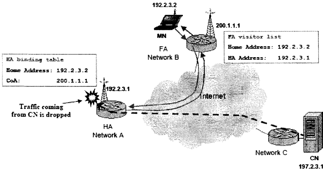
Fig. 3.7, IPv4 MN Moves to FA [OPN]
