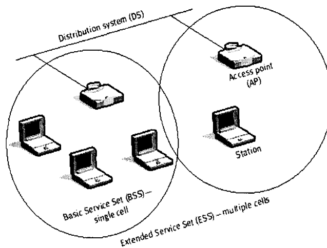
Fig. 3.3, Infrastructure of the 802.11 WLAN
