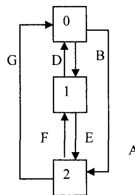
Fig. 2.7, Availability Model
