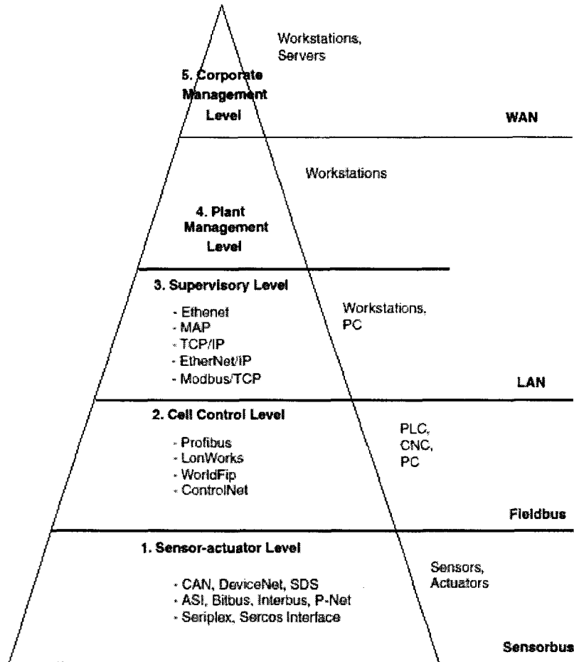
Fig. 2.3, A general network hierarchy model [LIA 01b]
