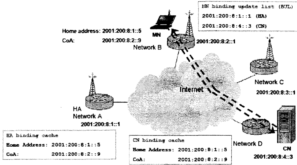
Fig. 3.12, IPv6 MN Performs Route Optimization with CN [OPN]
