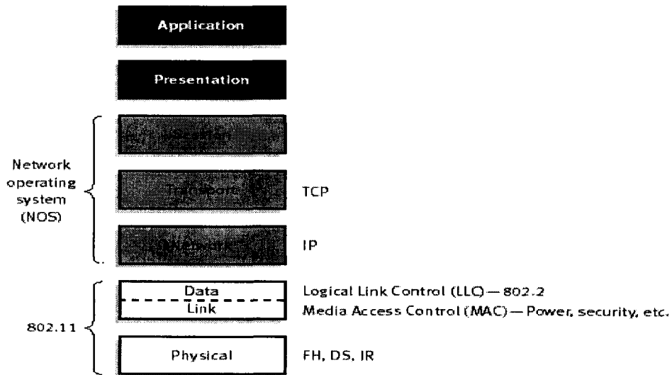
Fig. 3.2, Network Layers and Their Relation with WiFi
