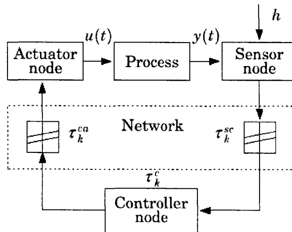
Fig. 2.2, NCS Block Diagram [NIL 98]
