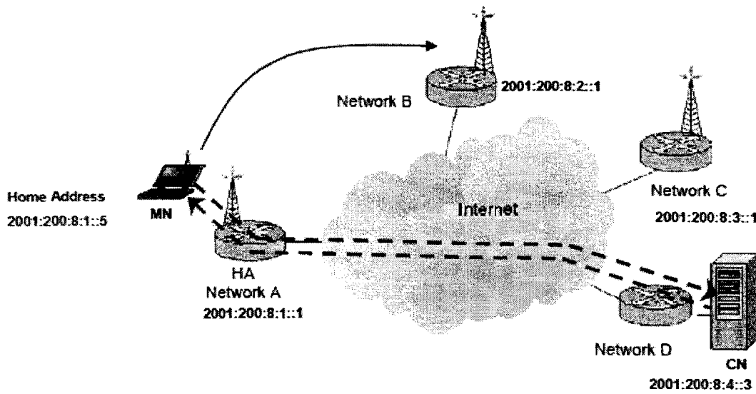
Fig.3.9, IPv6 MN at Home Network [OPN]
