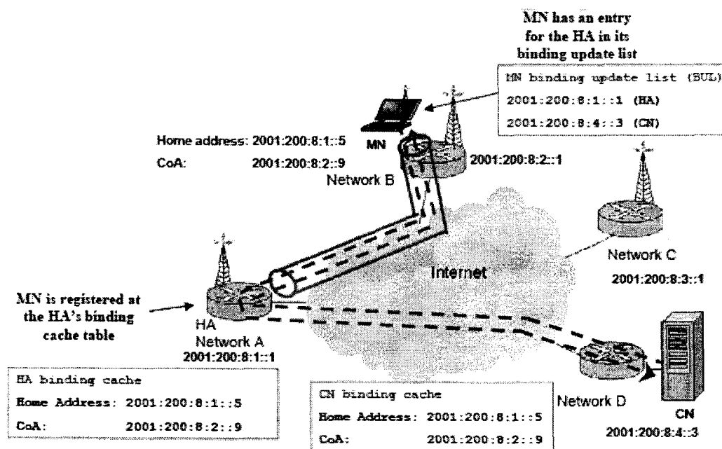
Fig.3.11, IPv6 MN Performs Tunnel with CN via HA [OPN]
