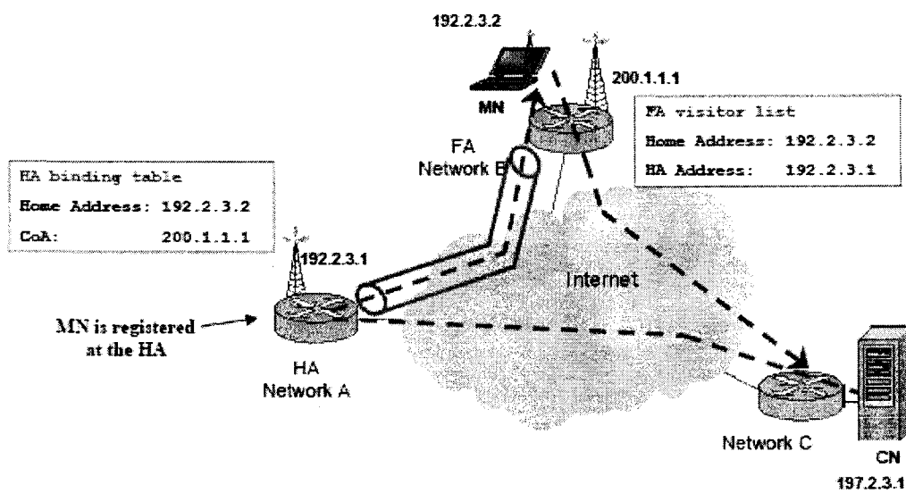
Fig. 3.8, IPv4 MN Establishes Tunnel at FA [OPN]
