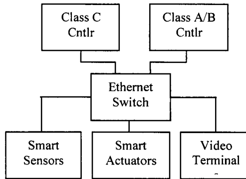
Fig. 2.14, Fault-Tolerant Vehicle On-Board Network Controllers
