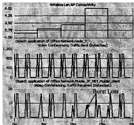
Fig. C, MN V=33Km/hr, MIPv4, t_{\text{packet}}=18\text{sec} , 3PB
