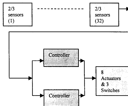
Fig. 2.12, RBD for TMR Configuration
