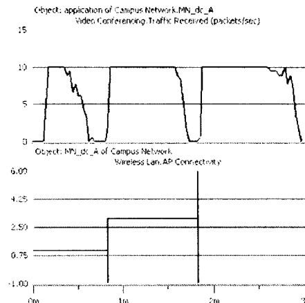
Fig. I, Traffic received in packets/second and AP connectivity for a mobile node moving at 33Km/hr in 802.11g architecture, transmit power 4mW
