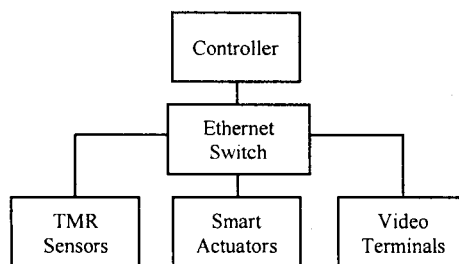
Fig. 2.15, TMR Vehicle On-Board Network Sensors
