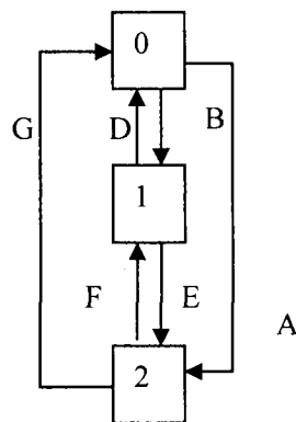
Fig. 2.7, Availability Model
