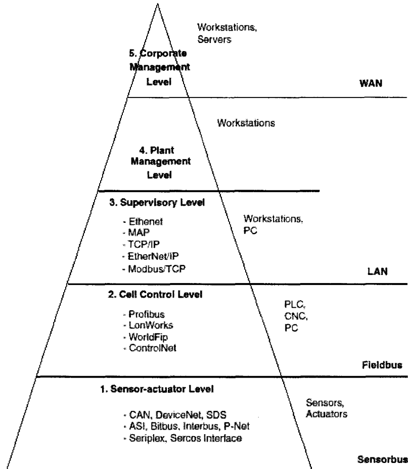
Fig. 2.3, A general network hierarchy model [LIA 01b]
