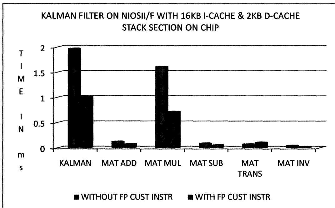
Figure 43: Effects of on chip and off chip memory sections on Kalman Filter
