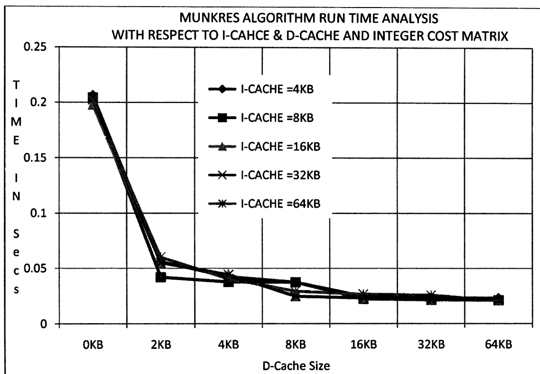
Figure 55: Cache Behavior for Munkres Algorithm with Integer Cost Matrix
