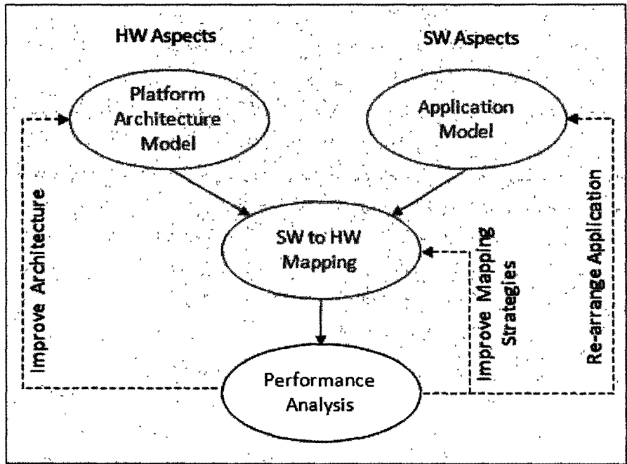
Figure 37: Performance Analysis and Optimization
