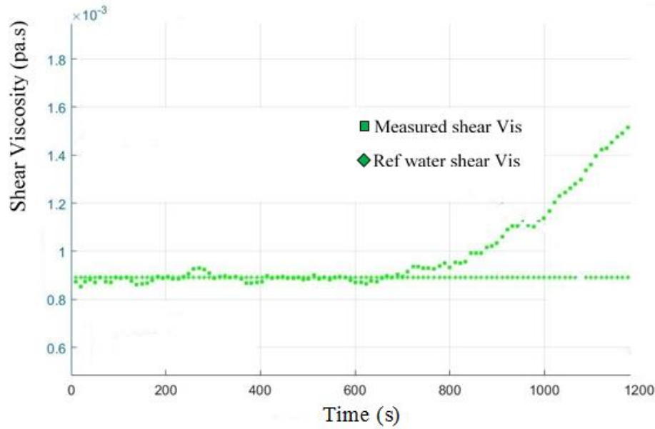
Figure II.30. Shear viscosity variation during the evaporation of 4% C_v Au-water nanofluid droplet on a silicon substrate at room temperature.
