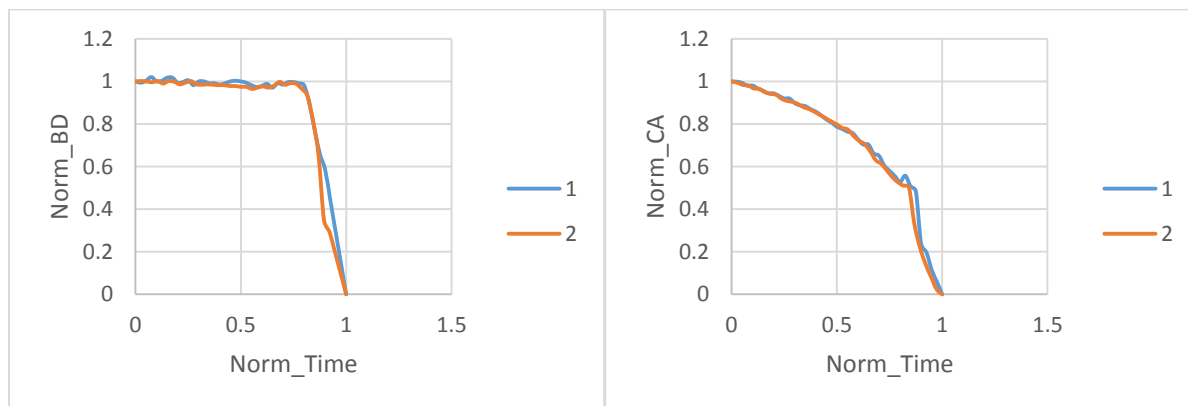
Figure 2. The repeatability of the contact angle and base diameter variations of 2nm citrate-PBS gold/ water droplet at 77 °C surface temperature.
