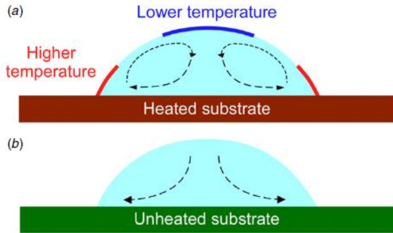
Figure I.6. (a) Liquid flow patterns in an evaporating droplet on a heated substrate. A stable Marangoni flow forms in the droplet. (b) Liquid flow patterns in an evaporating droplet on an unheated substrate. Evaporation induced radial flow is the dominant flow. [62]
