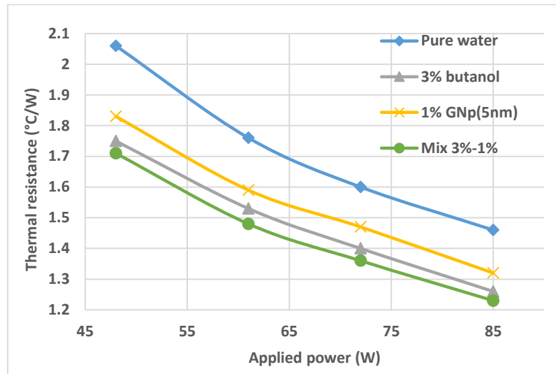
Figure IV.5. Thermal resistance for water, butanol self-retetting and gold nanofluids.
