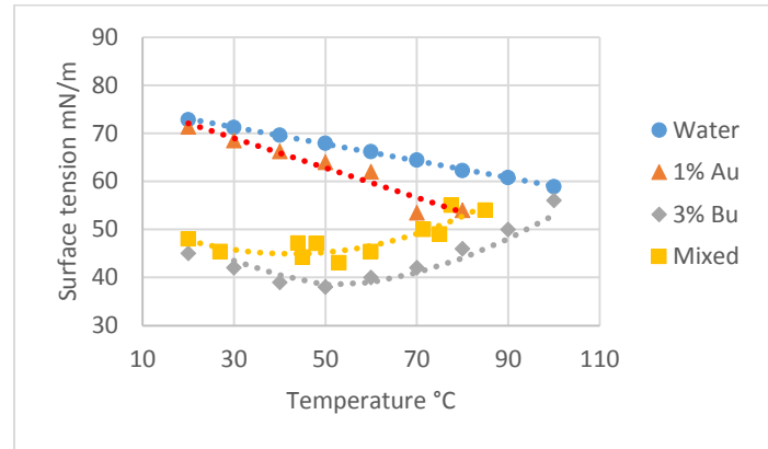
Figure IV.7. Surface tension measurements for water, butanol (3% C_v ), gold (1% C_v ), and a mixture of butanol self-wetting gold nanofluid (Bu 3%-Au 1% C_v ) using KRUSS Pendant method.
