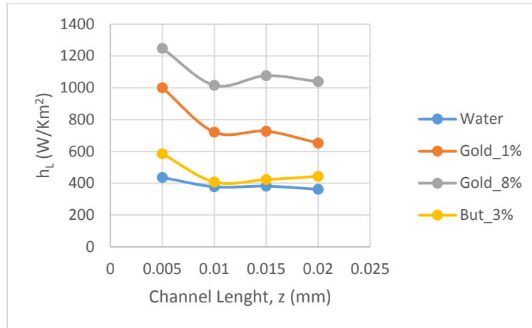
(a) P_1 = 2.41 \text{ W}
