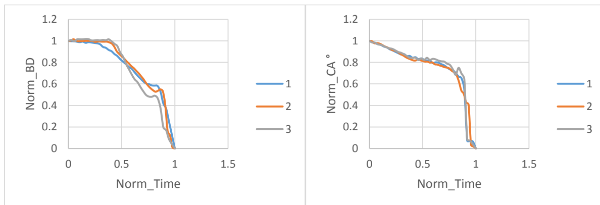
Figure 1. The repeatability of the Contact angle and base diameter variations of pure water droplet at 77 °C surface temperature.
